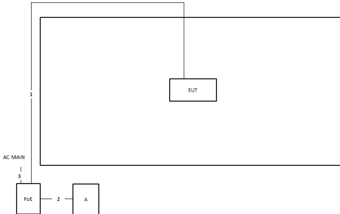
Test Setup Diagram - Transmitter Spurious Emissions above 1 GHz
