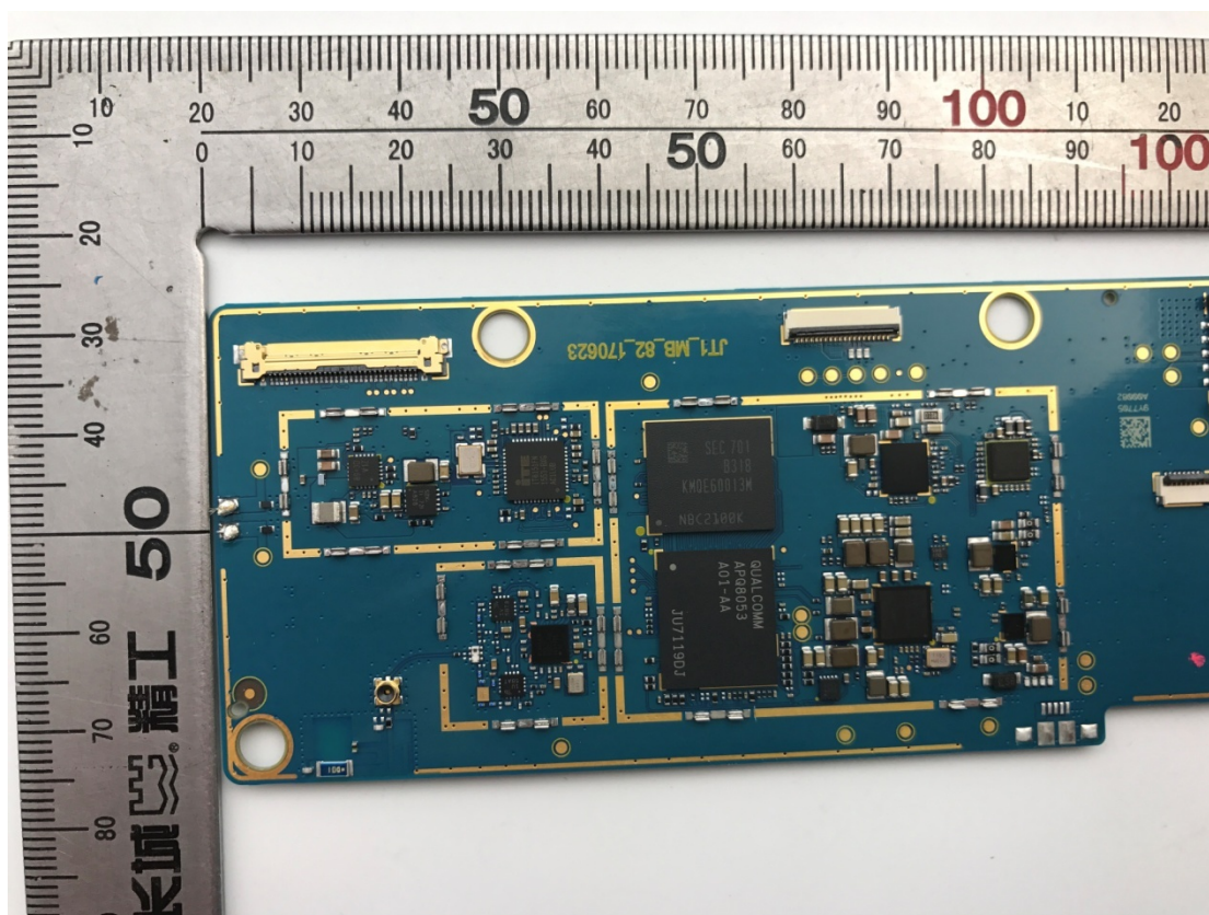
Main board close shot
