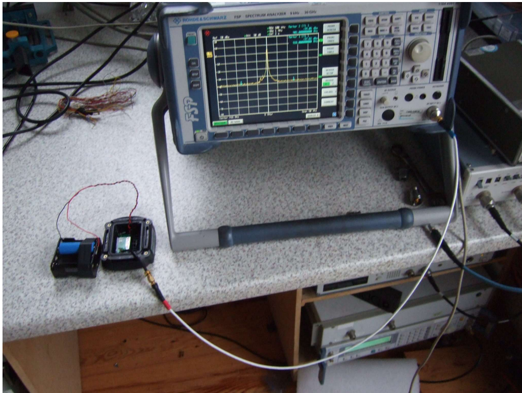
Figure 2: Conducted Power Measurements
