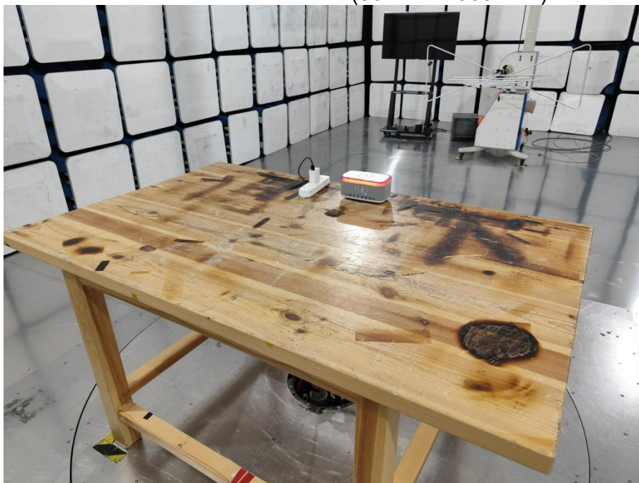
Radiation Emission Test (30MHz~1000MHz)
