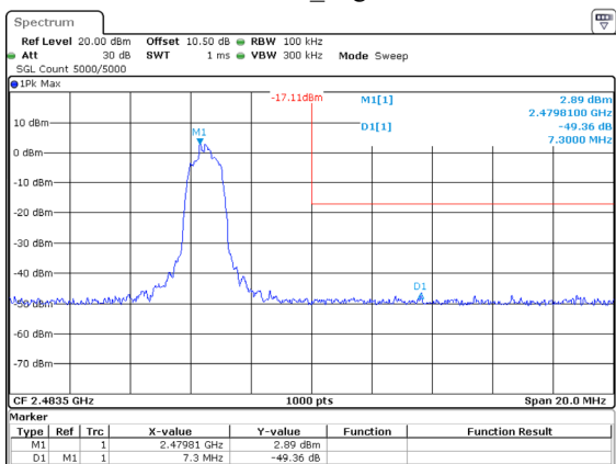
2DH1_High
