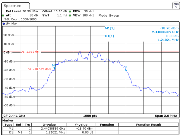
3DH1_Middle
