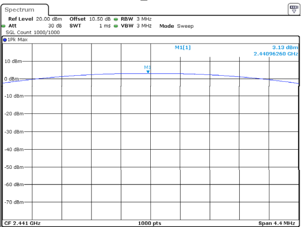
DH1_Middle
