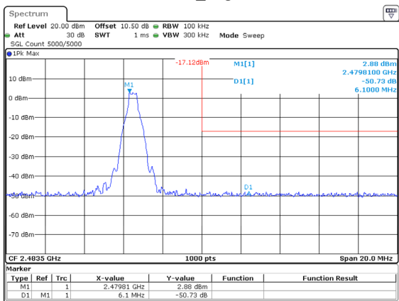
DH1_High
