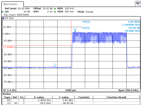
DH1_Hopping_Lower
