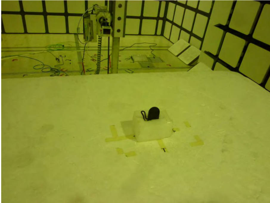
18 GHz~26.5 GHz _ Rear View
