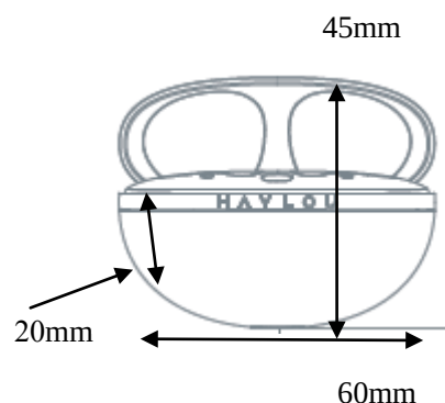
Charging Box
