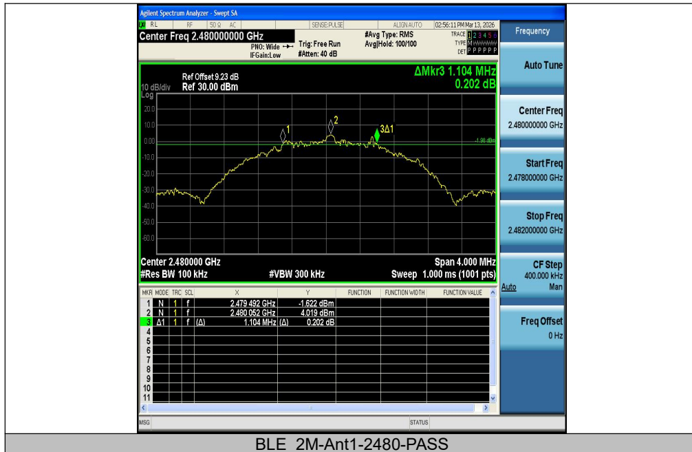
BLE_2M-Ant1-2480-PASS Test Graphs of DTS Bandwidth
