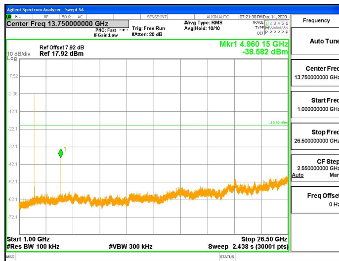
BLE_2Mbps_Ant1_2480_1000~26500
