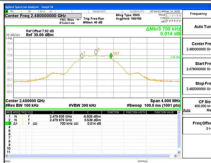
BLE_1Mbps_Ant1_2480
