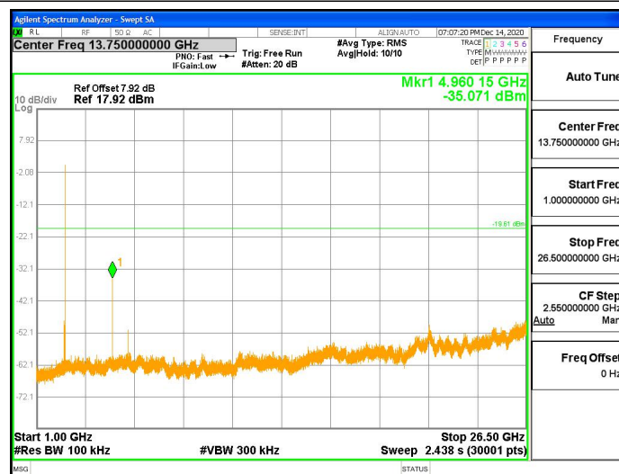
BLE_1Mbps_Ant1_2480_1000~26500
