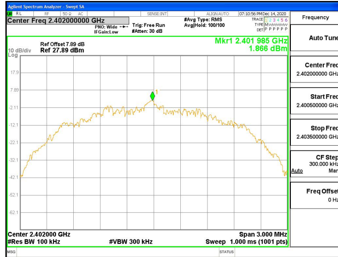
BLE_2Mbps_Ant1_2402_30~1000
