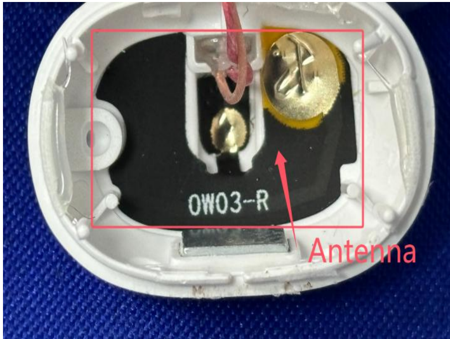
View of Product-5 R-ear
