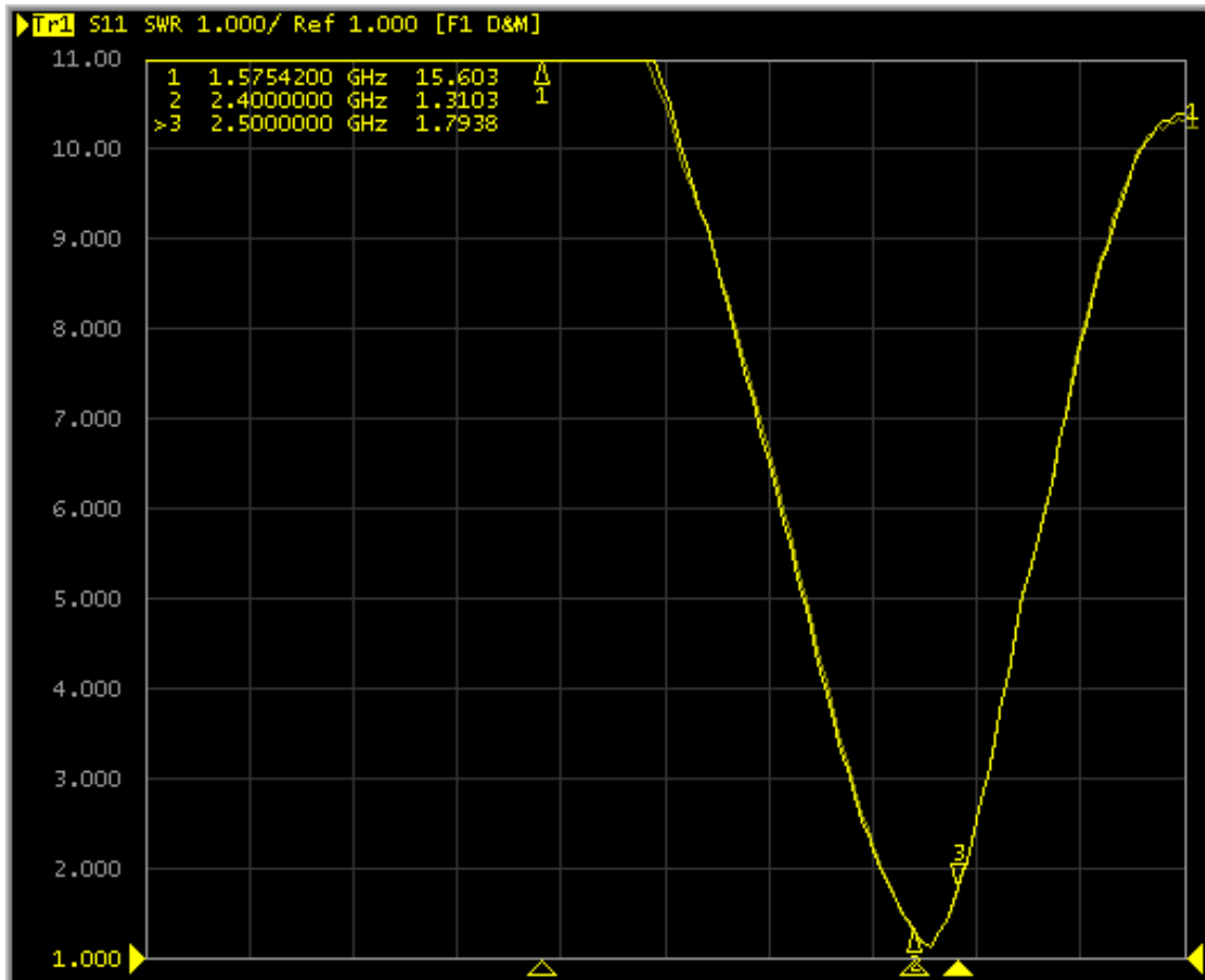
Return SWR
