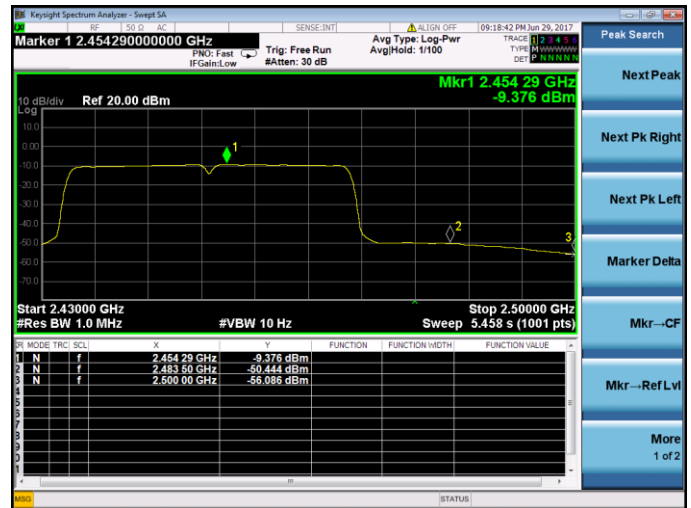
802.11n-HT40-High channel(Average)
