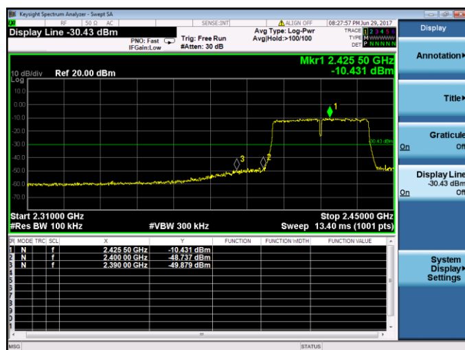
802.11n-HT40-Low channel
