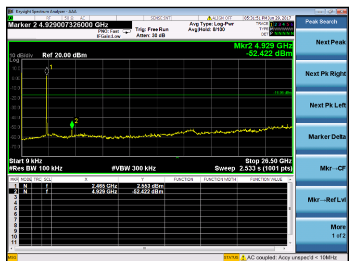
802.11b-High channel
