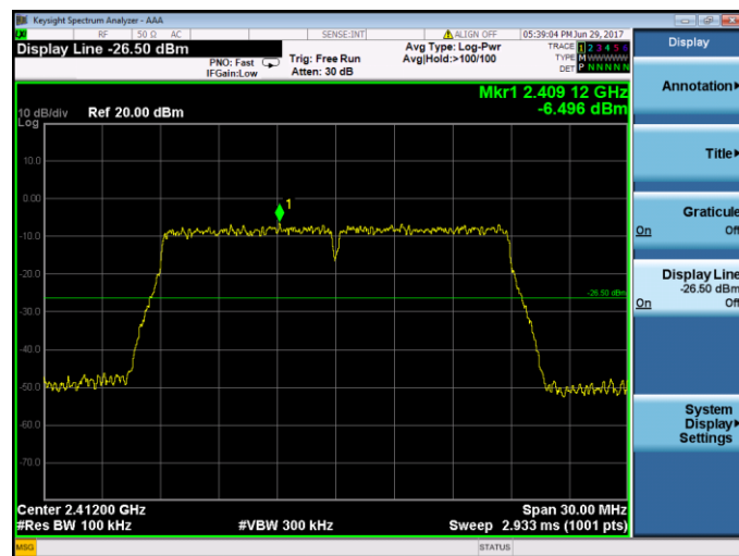
IEEE 802.11n HT20-Channel 1 / 2412 MHz
