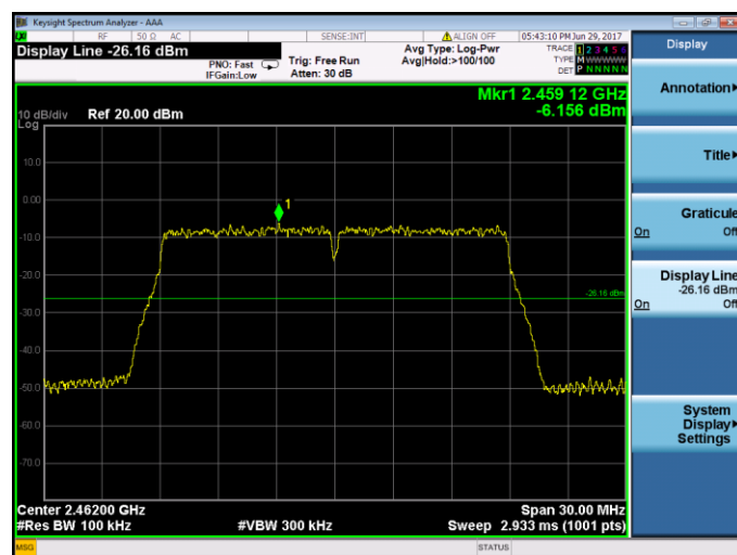
IEEE 802.11n HT20-Channel 11 / 2462 MHz
