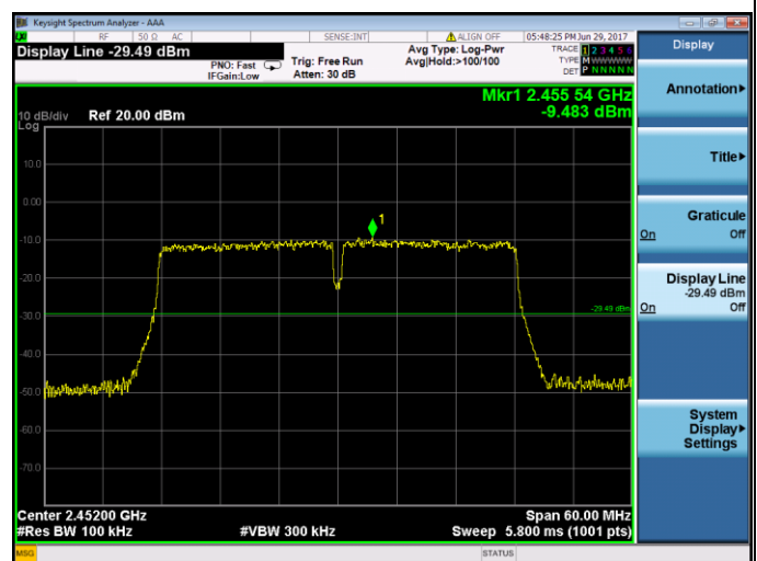
IEEE 802.11n HT40-Channel 9 / 2452 MHz
