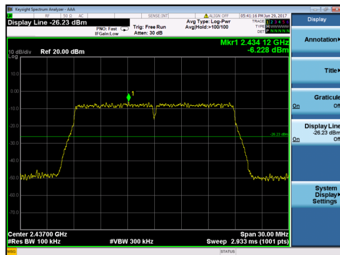
IEEE 802.11n HT20-Channel 6 / 2437 MHz
