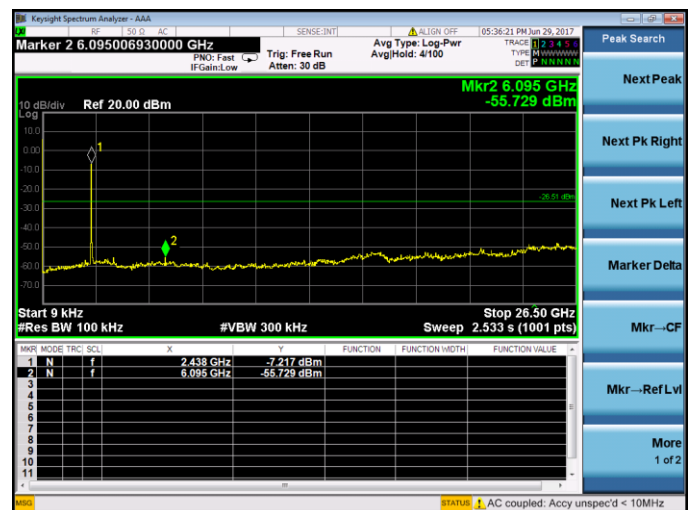
802.11g-Middle channel
