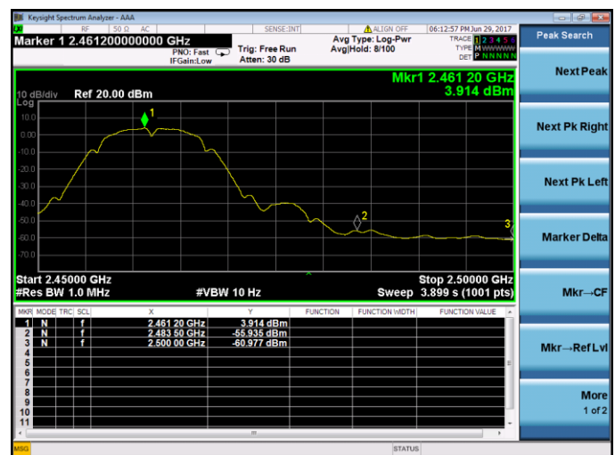
802.11b-High channel(Average)
