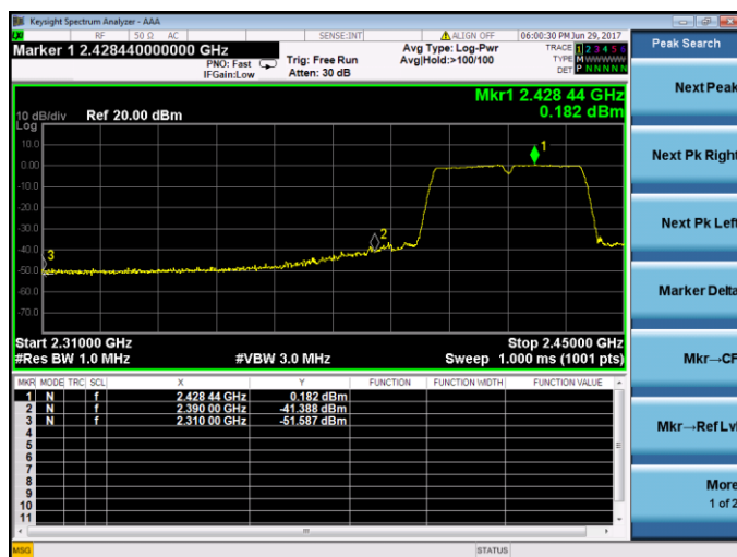
802.11n-HT40-Low channel(Peak)
