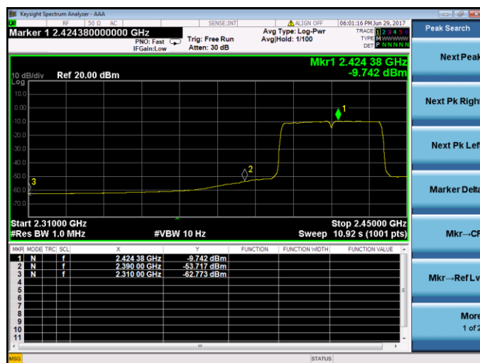
802.11n-HT40-Low channel(Average)
