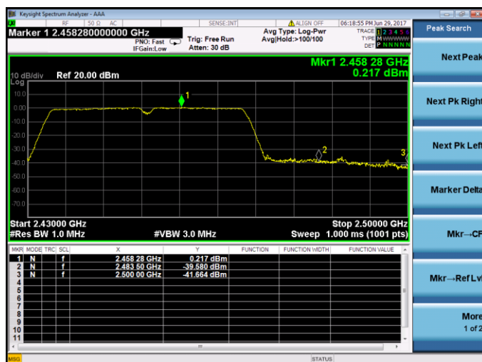
802.11n-HT40-High channel(Peak)
