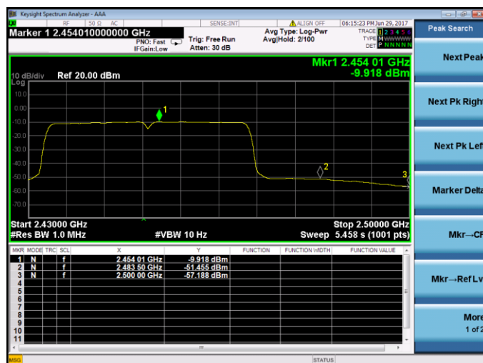
802.11n-HT40-High channel(Average)
