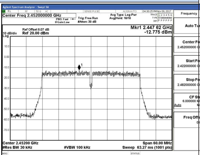
802.11n-HT40 High channel
