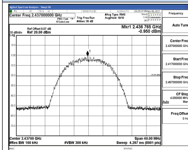
802.11b Middle channel Reference
