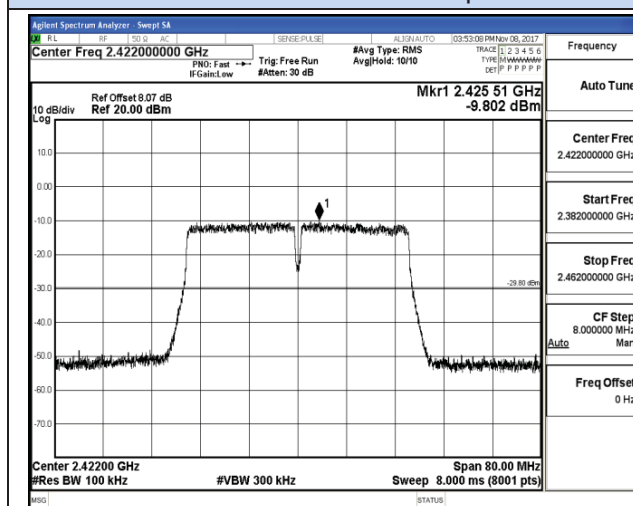
802.11n-HT40 Low channel Reference
