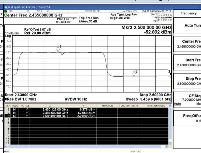
802.11n-HT40 High channel(Average)
