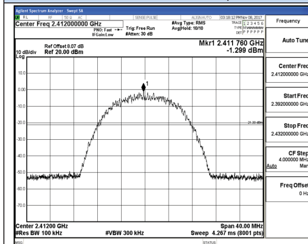
802.11b Low channel Reference
