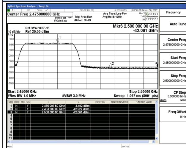
802.11n-HT20 High channel(Peak)
