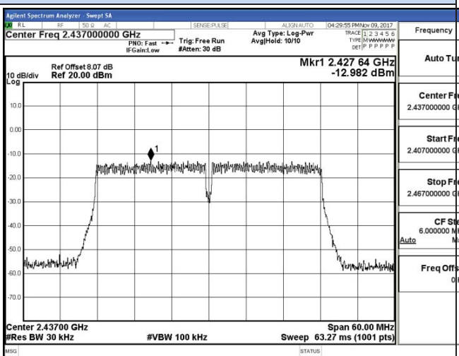
802.11n-HT40 Middle channel
