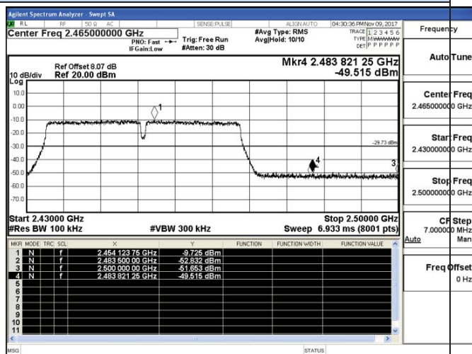
802.11n(HT40)-High channel
