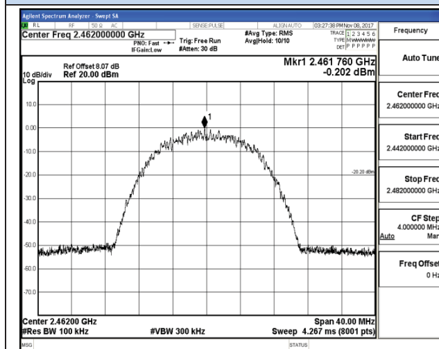
802.11b High channel Reference
