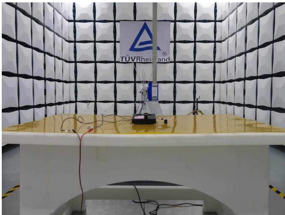
Test Setup Photo for Spurious Emissions (30 MHz-1 GHz)
