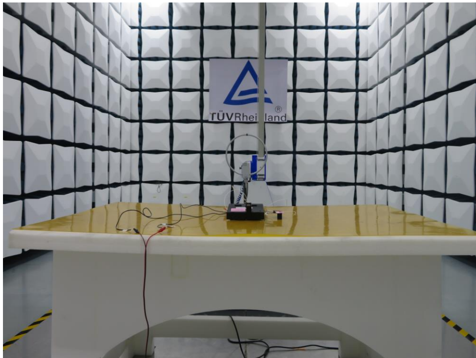
Test Setup Photo for Spurious Emissions (9 kHz-30 MHz)
