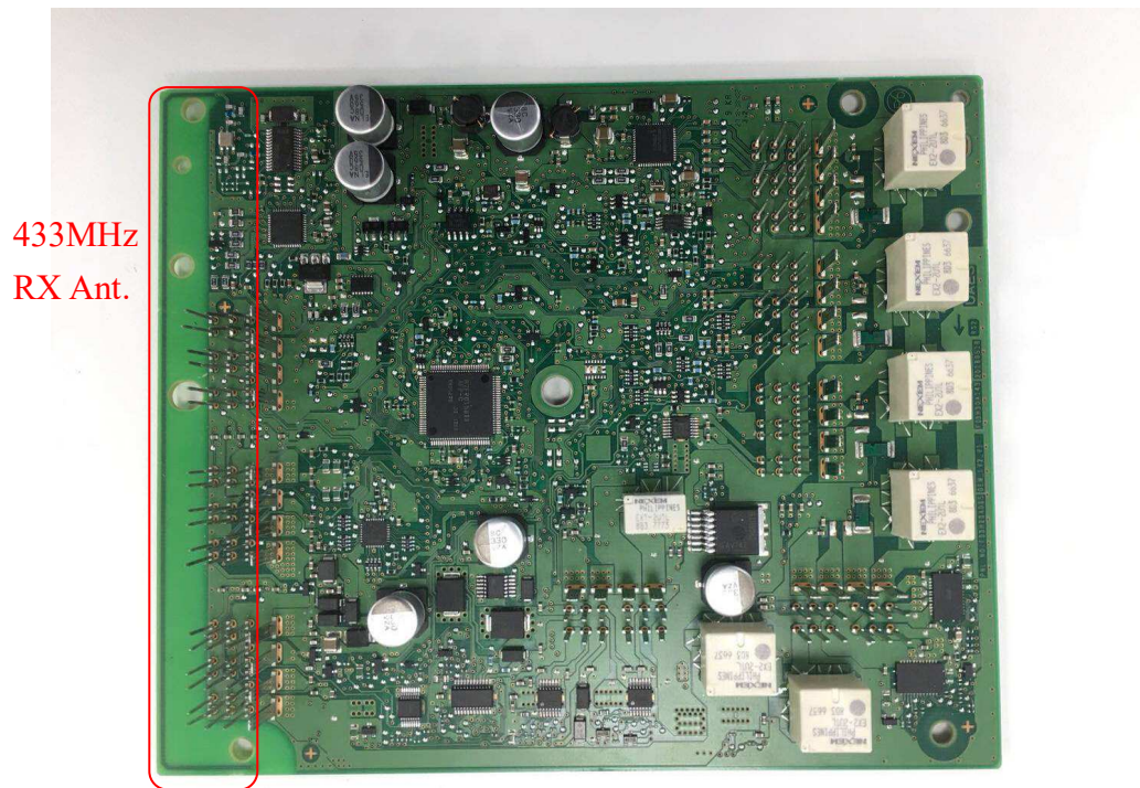
(1) EUT Photo
