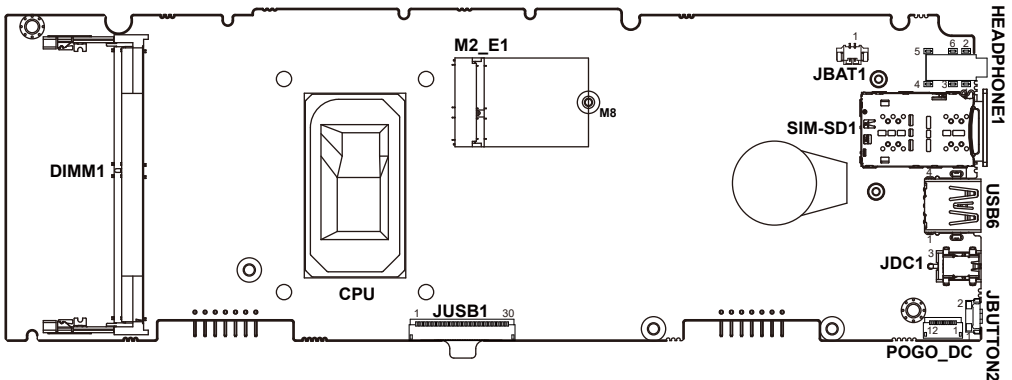
Figure 3-1. MB-T01T Main Board Component Locations (Top View)
