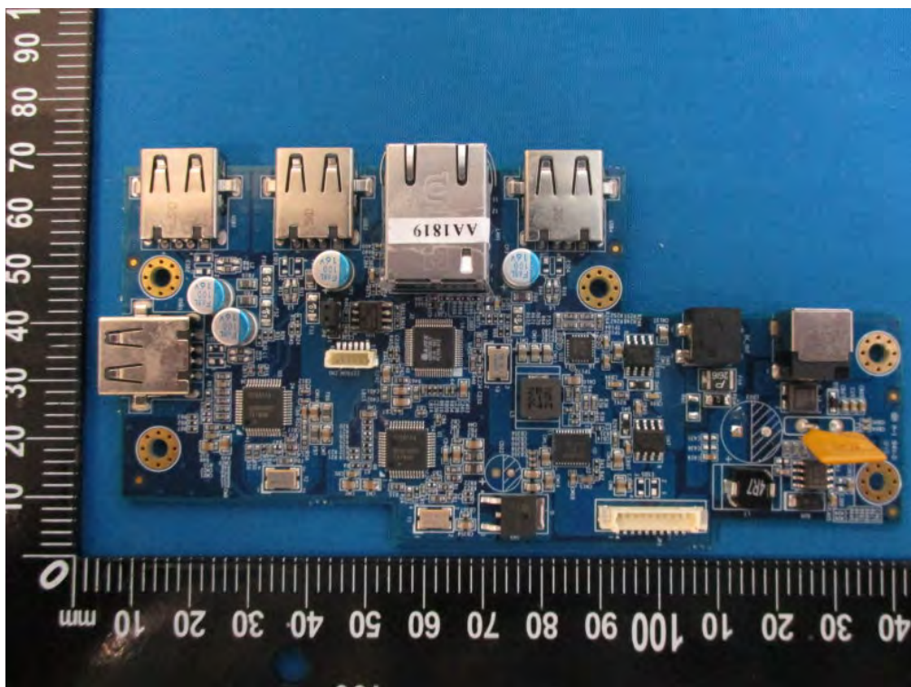
White Cradle - Main Board Top View
