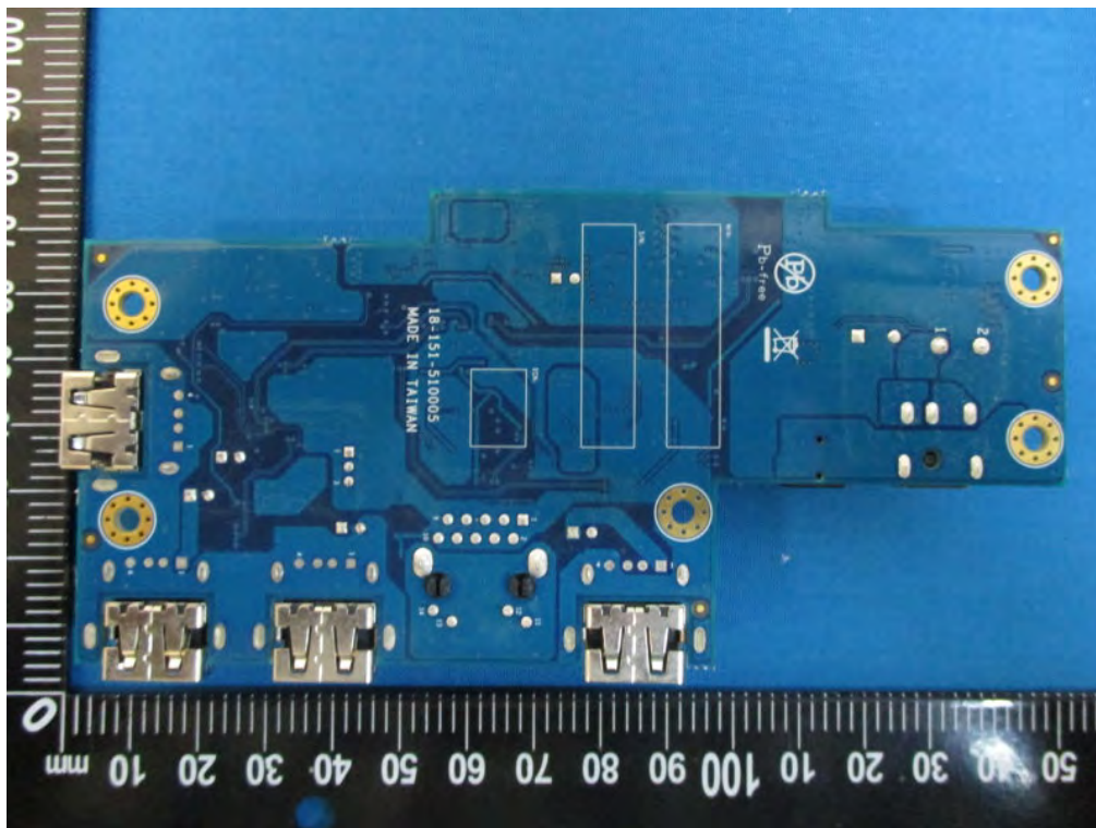
White Cradle - Main Board Bottom View
