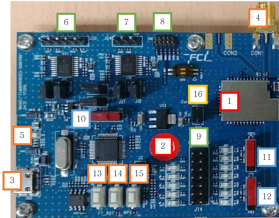
Figure 1.FCM9000S Module Board
