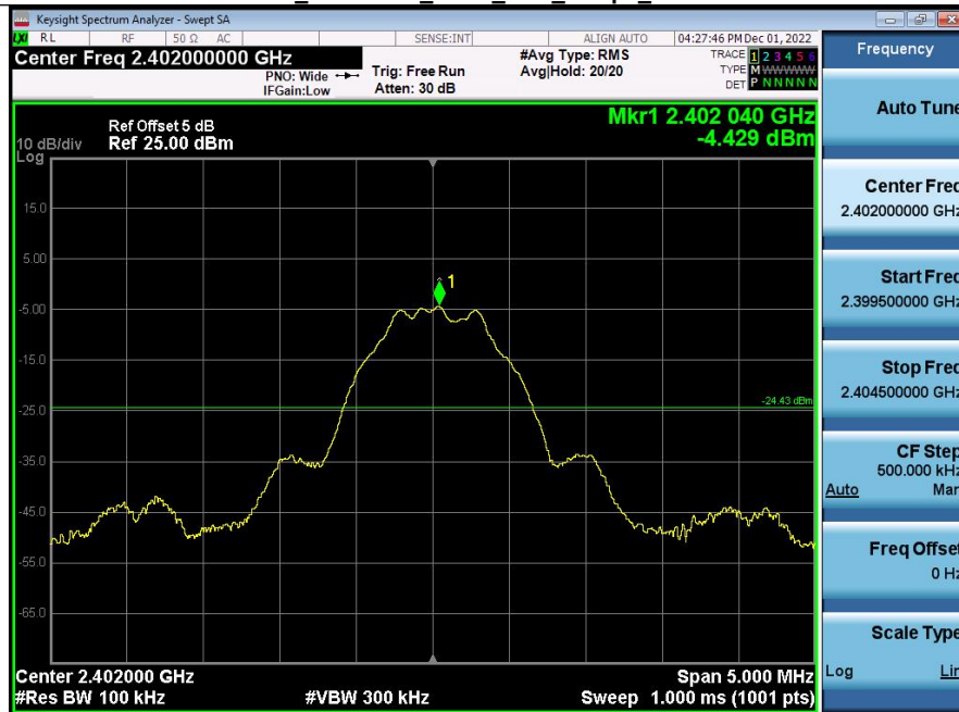
2_Spurious_Emission_BLE_1Mbps_2402
