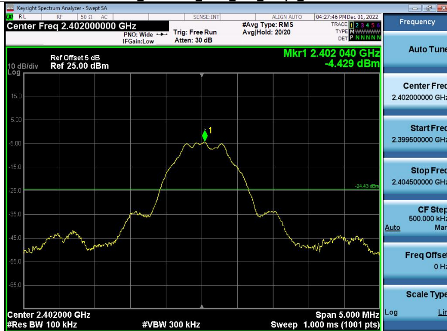
2 Bandedge_BLE_1Mbps_2402
