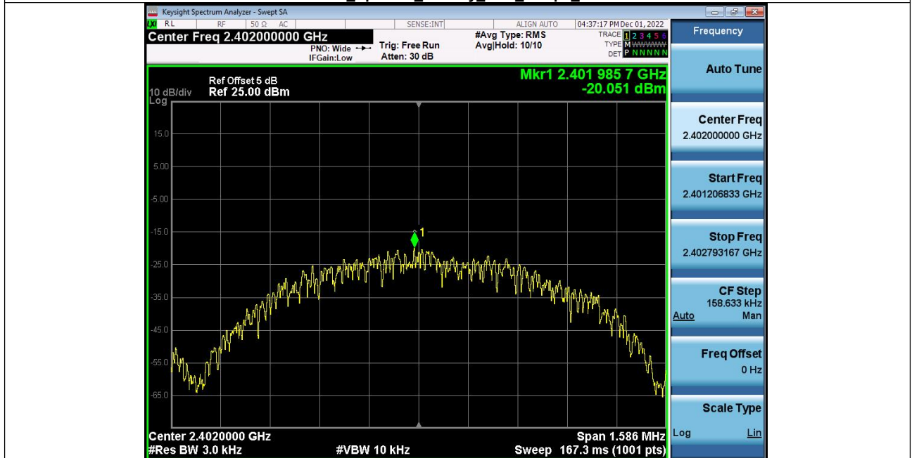
Power_Spectral_Density_BLE_1Mbps_2402
