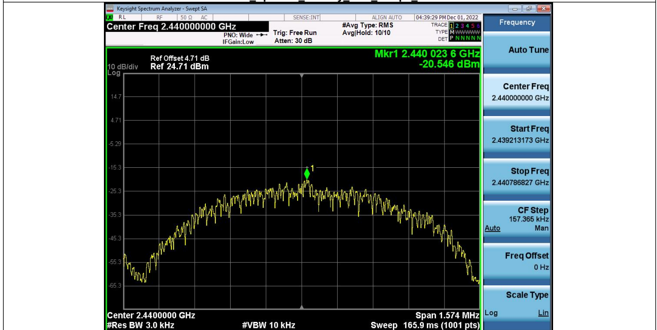
Power_Spectral_Density_BLE_1Mbps_2440
