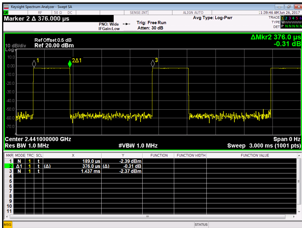
39 Channel @ DH1
