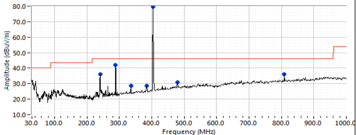
30 - 1000 MHz low channel @ 2443MHz
