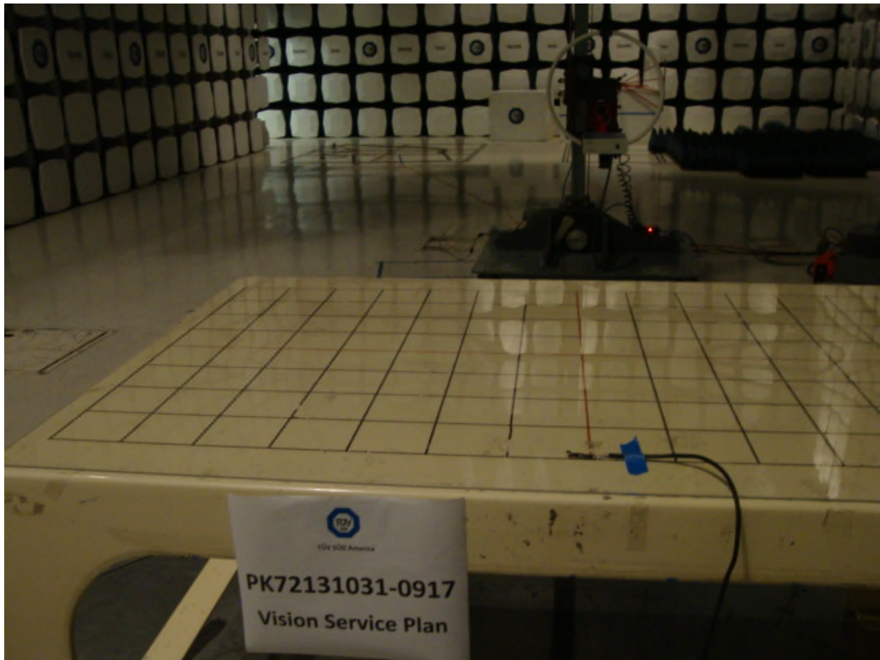
Radiated Emissions Test Setup (below 30MHz)
