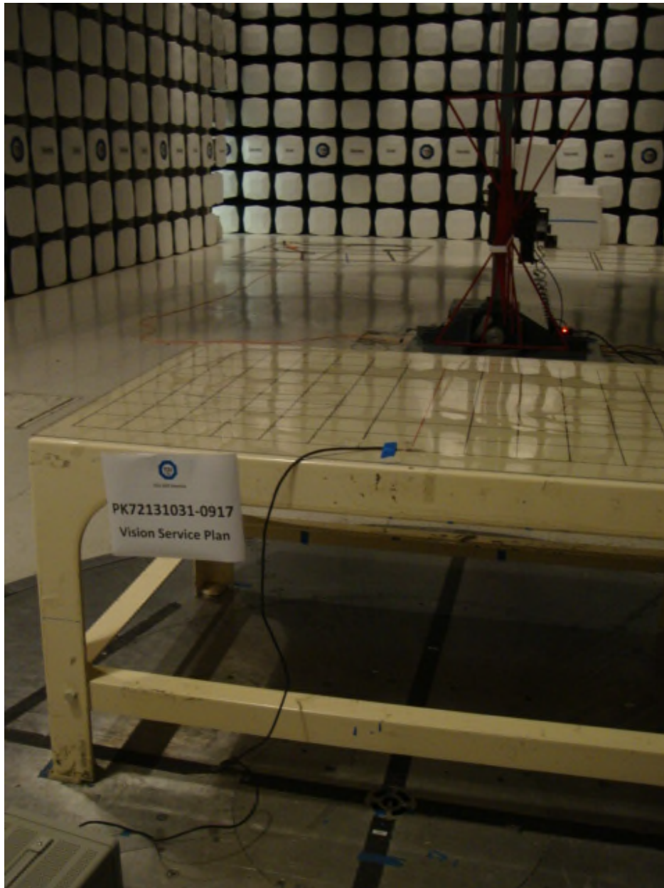
Radiated Emissions Test Setup (below 1GHz)
