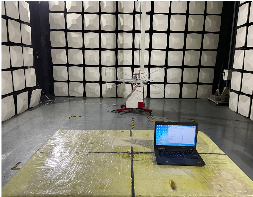
Radiated emission (30-1000MHz)
