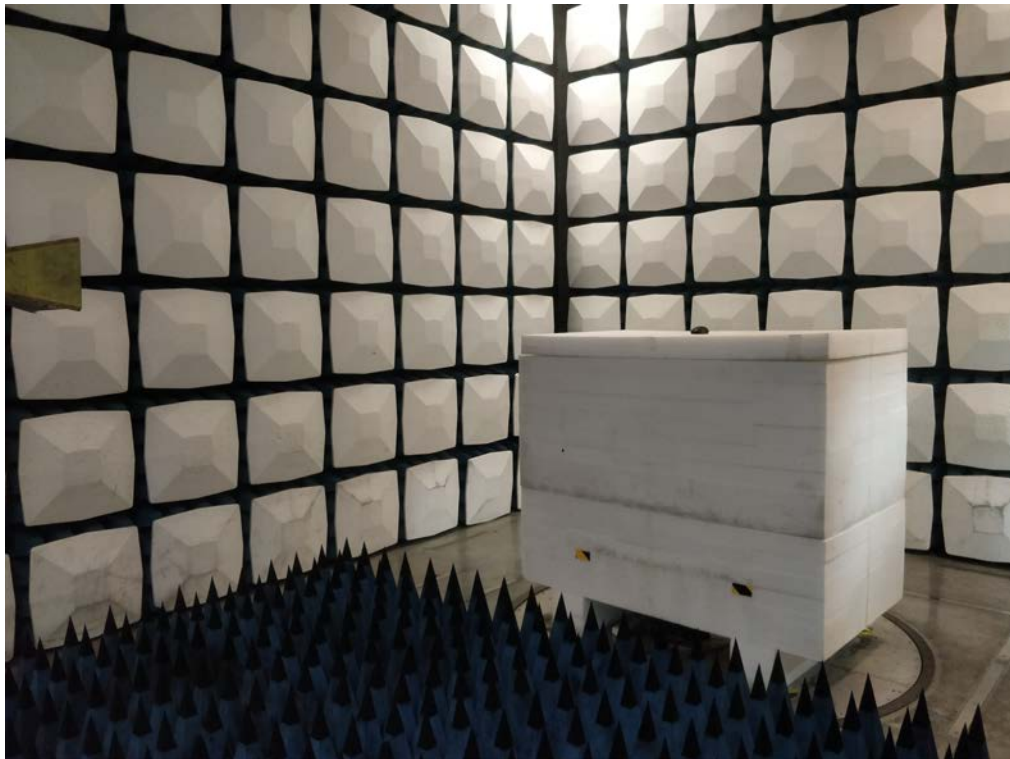
Radiated Emission Below 1GHz front View
