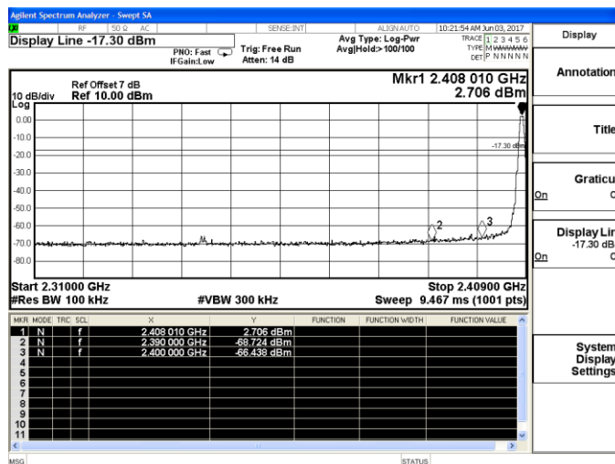
Channel 1 / 2408 MHz
