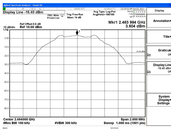
Channel 3 / 2464 MHz
