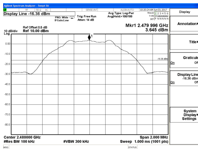
Channel 4 / 2480 MHz
