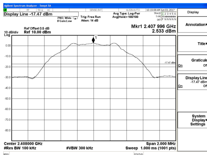
Channel 1 / 2408 MHz
