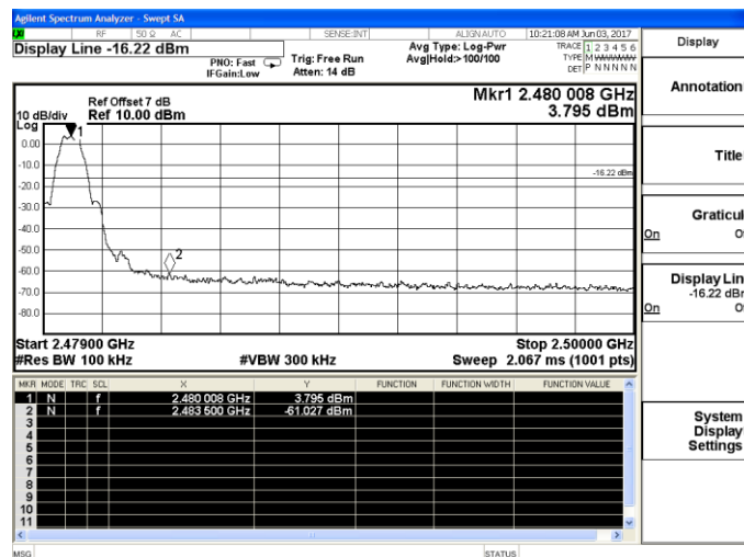
Channel 4 / 2480 MHz
