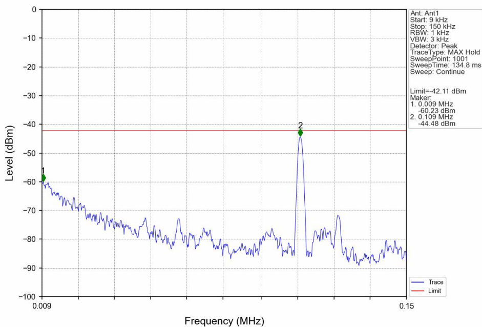
2.4G_LCH_2402MHz_Ant1_NTNV
