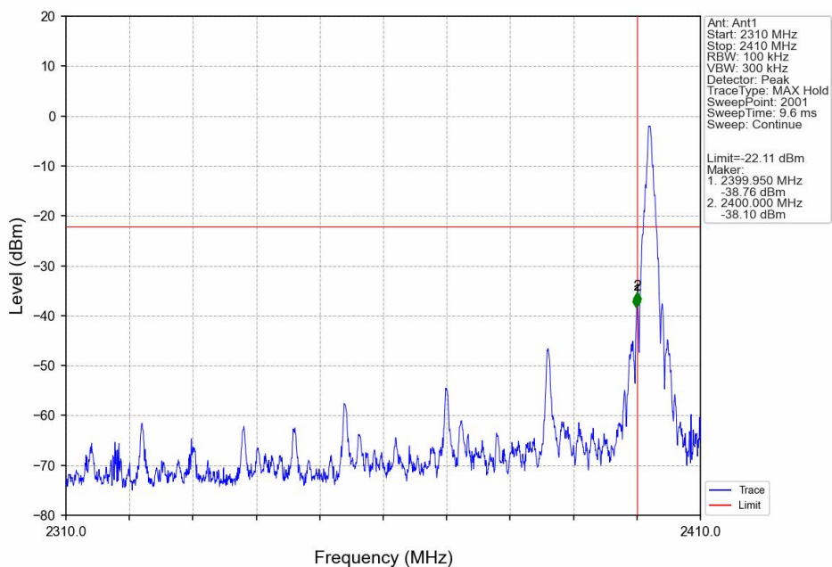
2.4G_LCH_2402MHz_Ant1_NTNV
