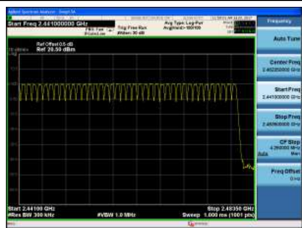
3-DH5(2Mbps)-2441~2483.5MHz
