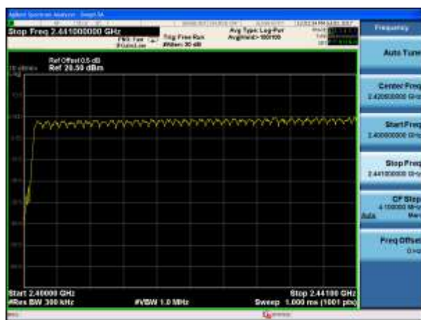
3-DH5(3Mbps)-2400~2441MHz
