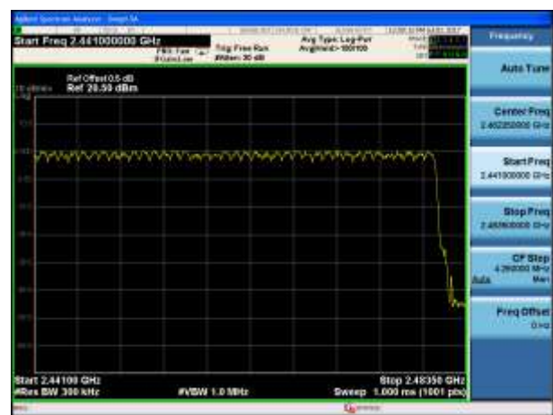
3-DH5(2Mbps)-2441~2483.5MHz
