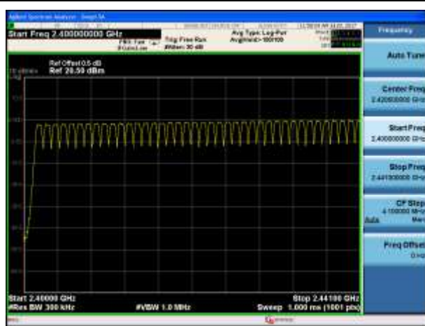
3-DH5(3Mbps)-2400~2441MHz
