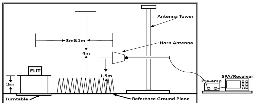
Above 1GHz
