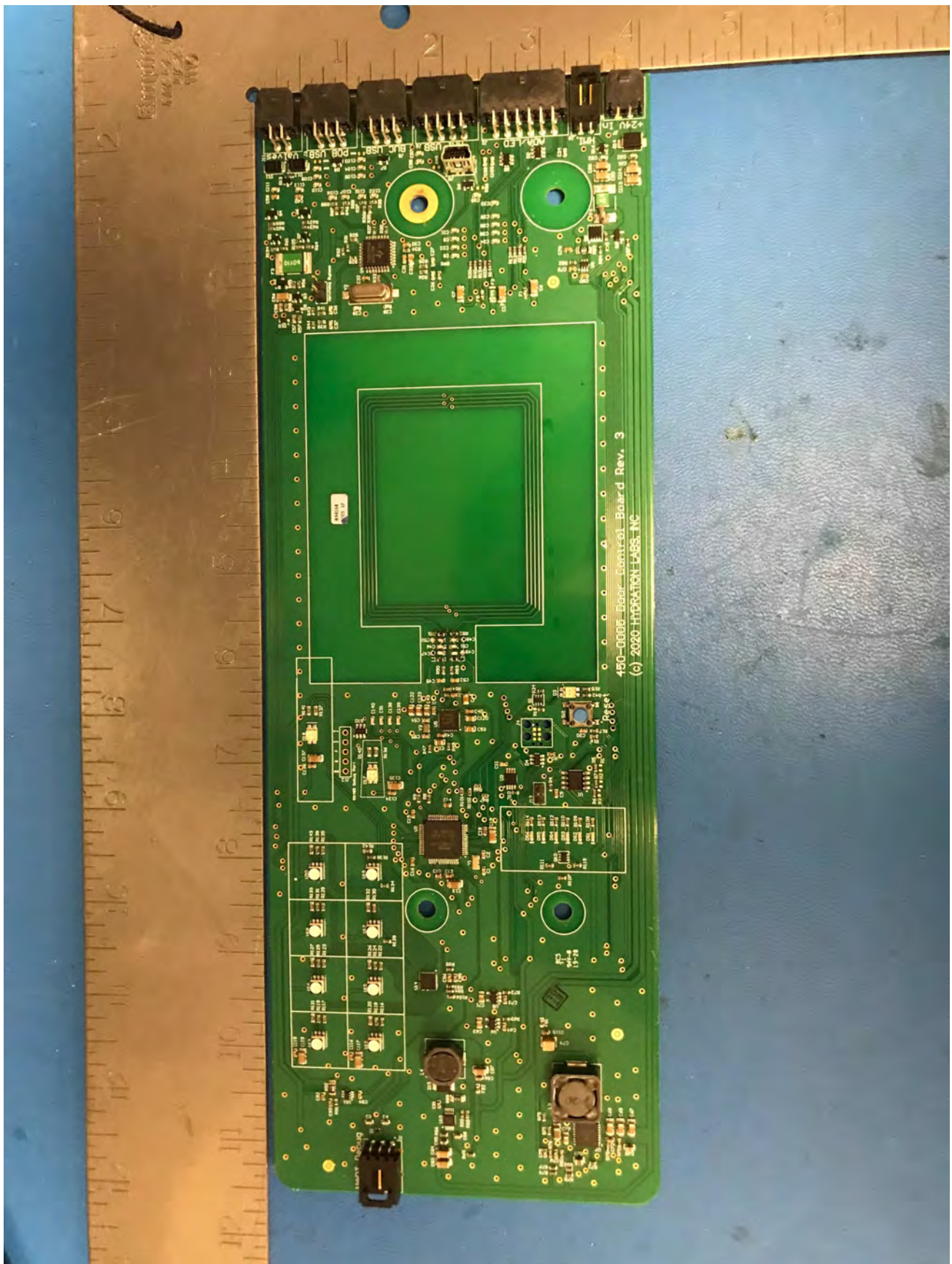
Door Control Board (RFID) TOP
