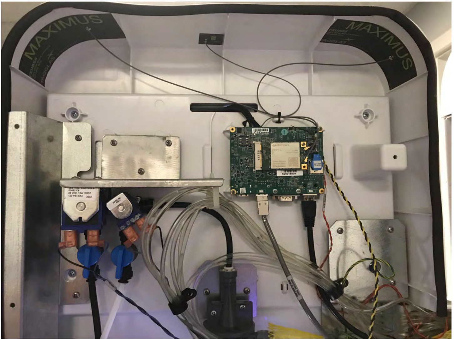
V2 Machine Inside Door View Closeup2
