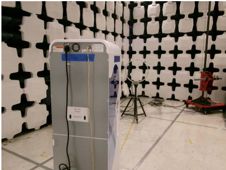
9k-30MHz Rear
