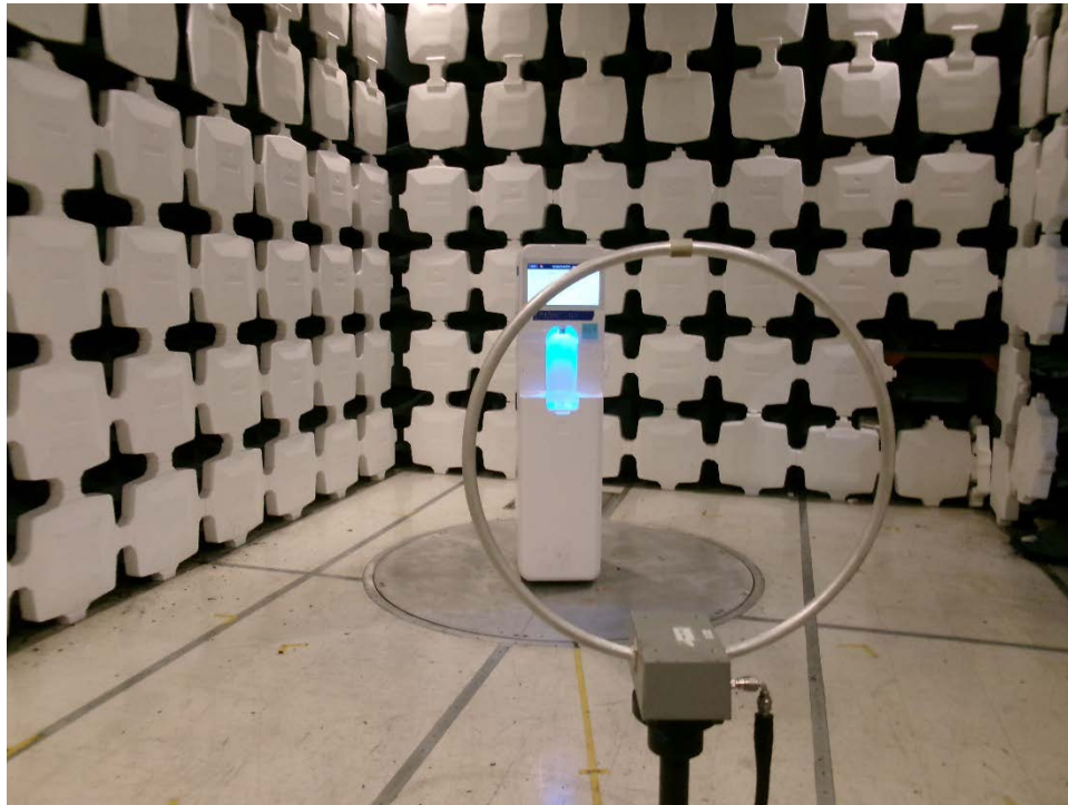
9k-30MHz Front
