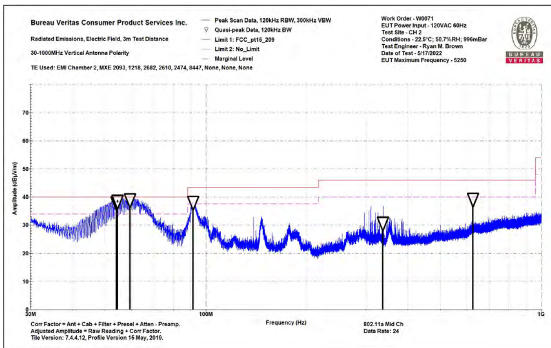
30-1000MHz Vertical
