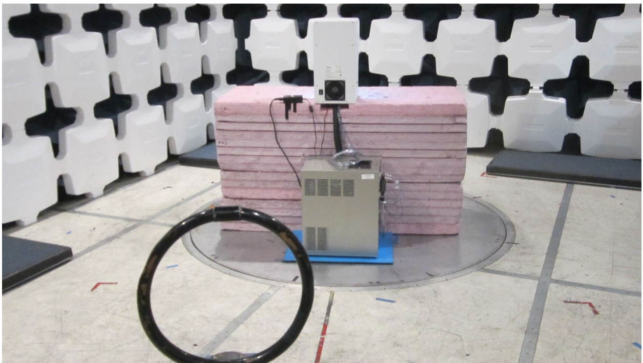
Radiated test setup, 9KHz – 30MHz
