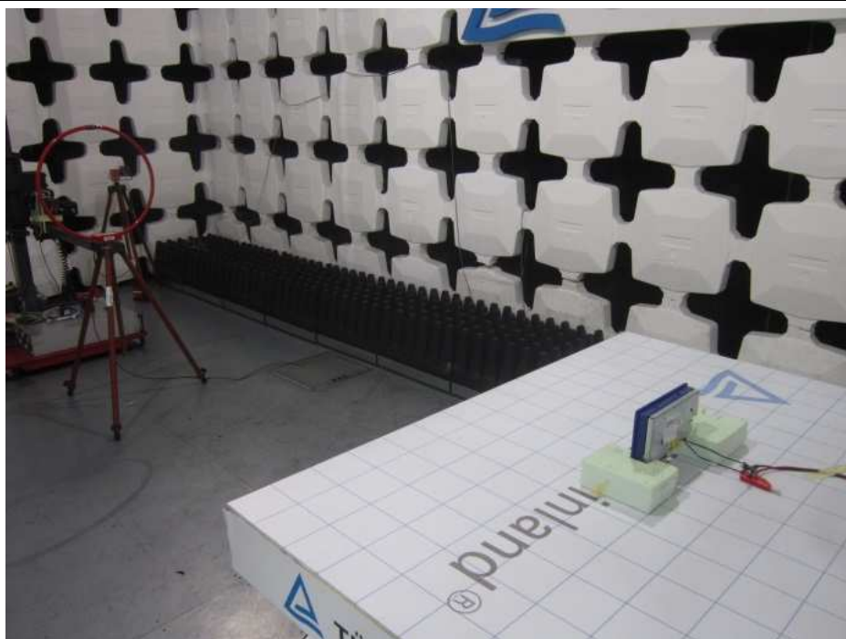
Set-up 9kHz-30MHz
