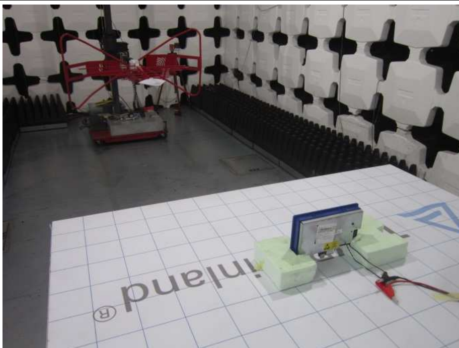
Set-up 30MHz-1GHz
