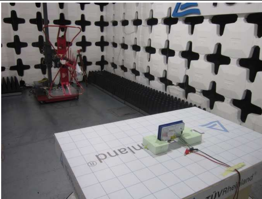
Set-up 30MHz-1GHz
