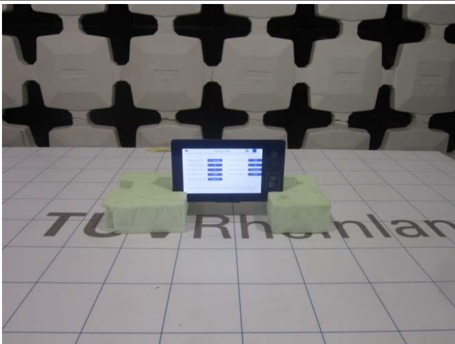
Set-up 30MHz-1GHz
