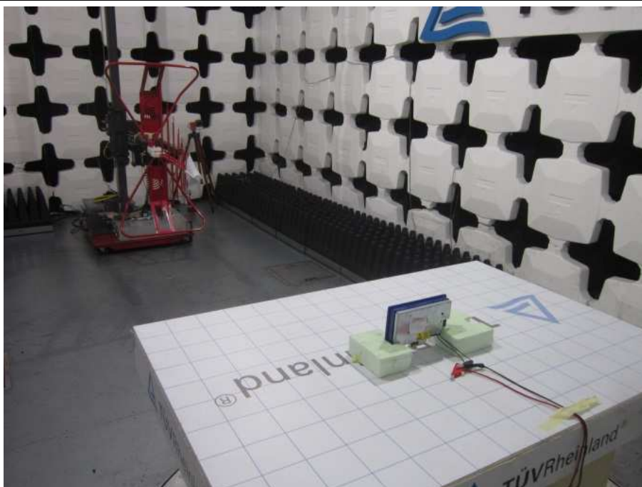
Set-up 30MHz-1GHz
