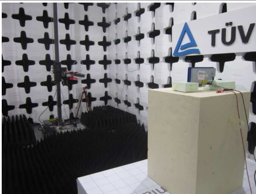
Set-up 1÷18GHz
