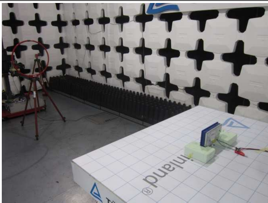
Set-up 9KHz-30MHz
