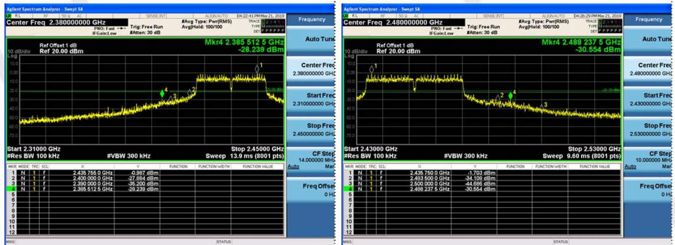
Left bandedge
