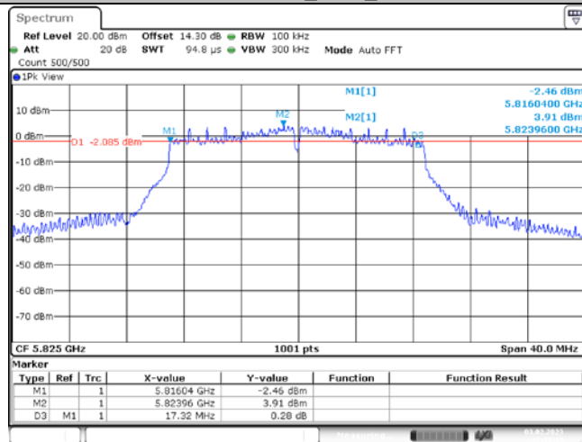
11AC20SISO_Ant1_5825
