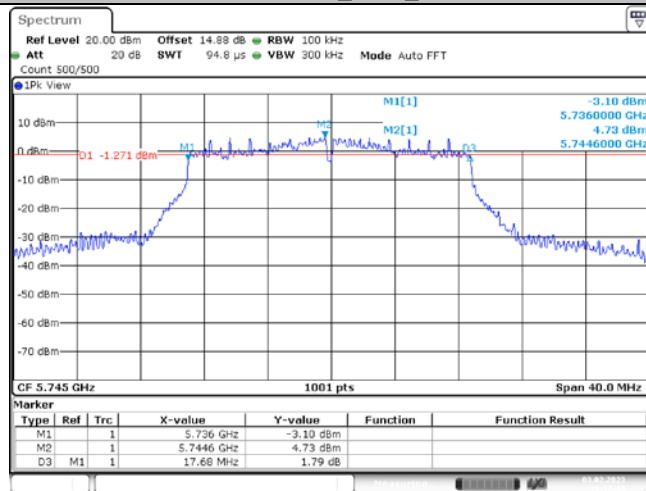
11AC20SISO_Ant1_5745
