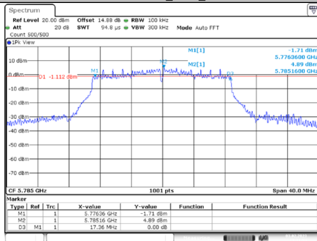
11AC20SISO_Ant1_5785
