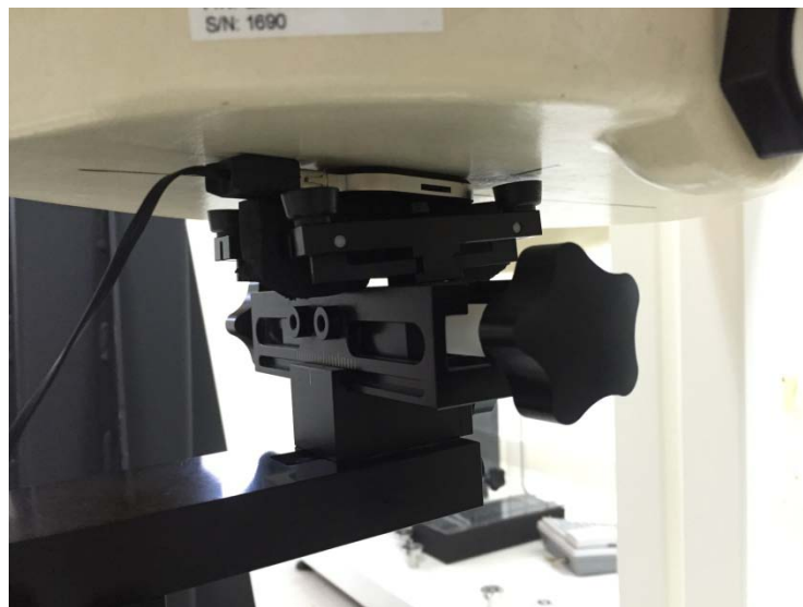
0mm Horizontal-Up Setup Photo
