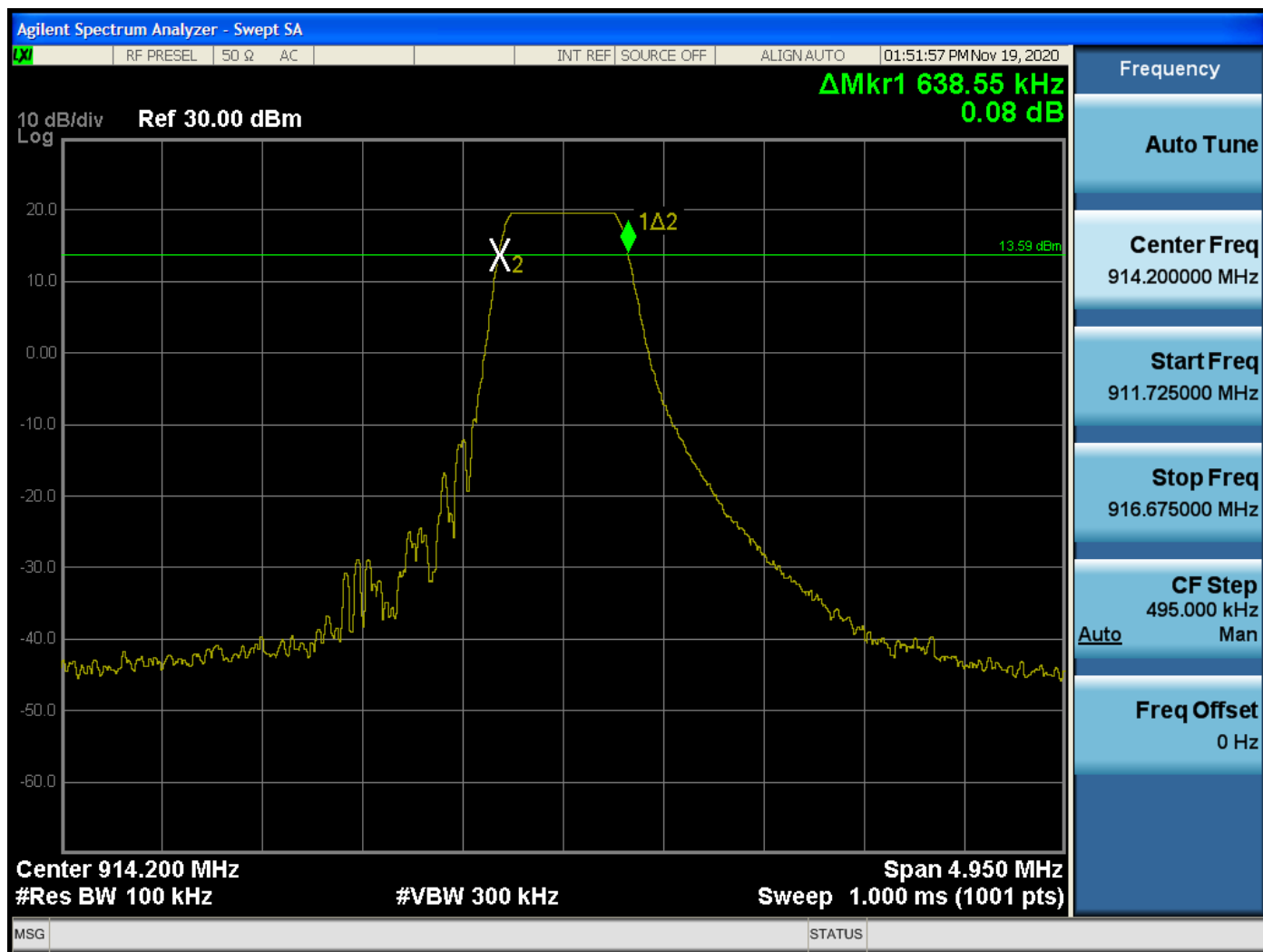
DTS Bandwidth – High Channel
