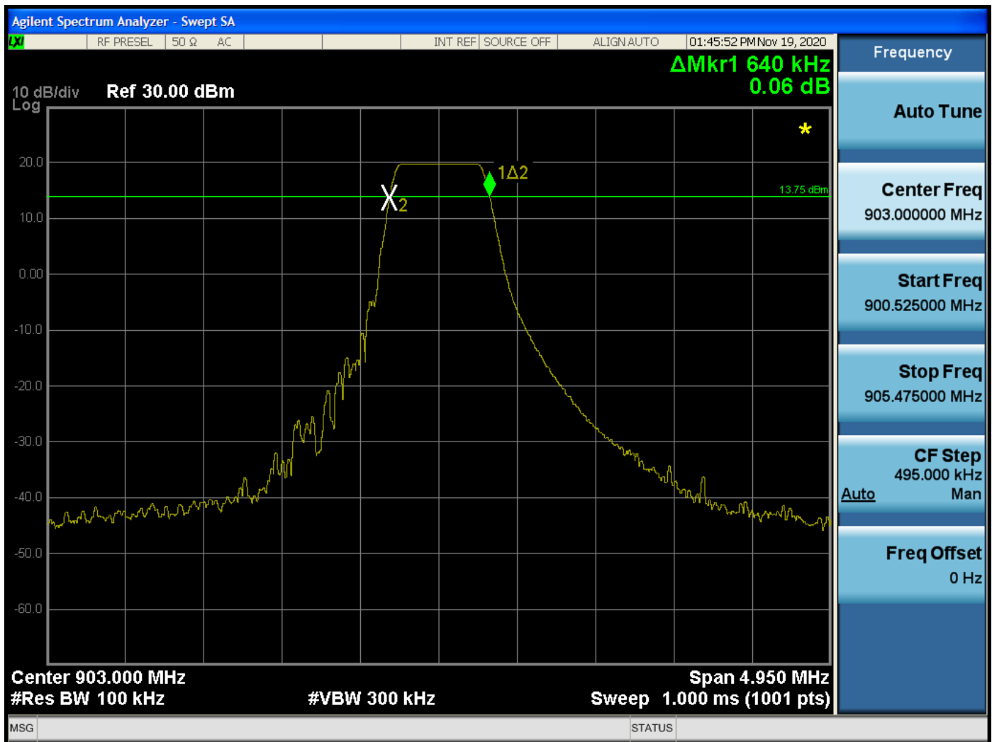
DTS Bandwidth – Low Channel
