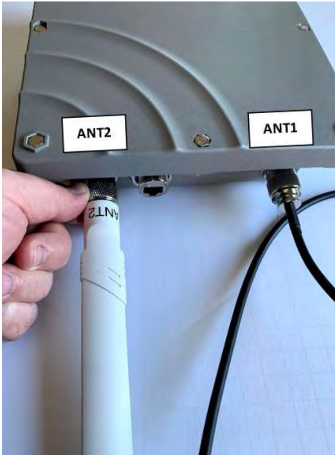
Figure 8: Connecting the Cellular antenna to the gateway
