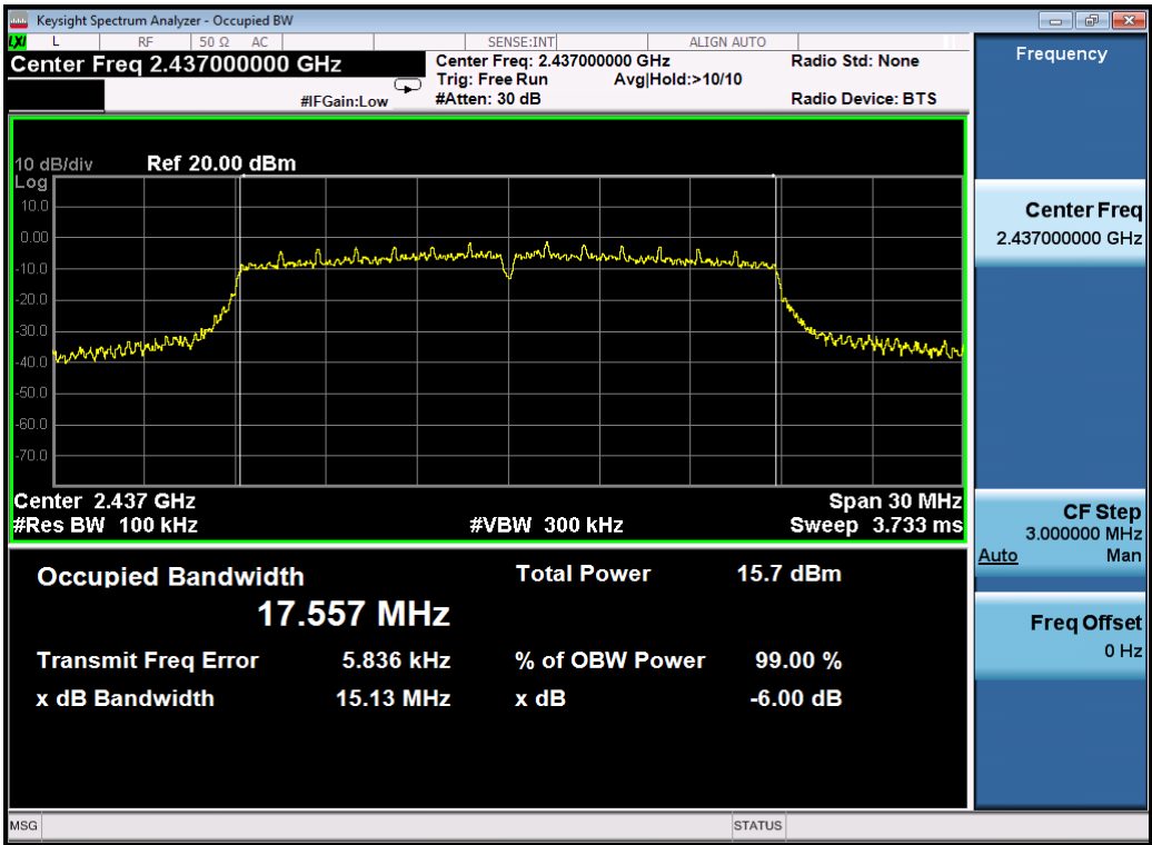
TEST PLOT OF BANDWIDTH FOR MIDDLE CHANNEL
