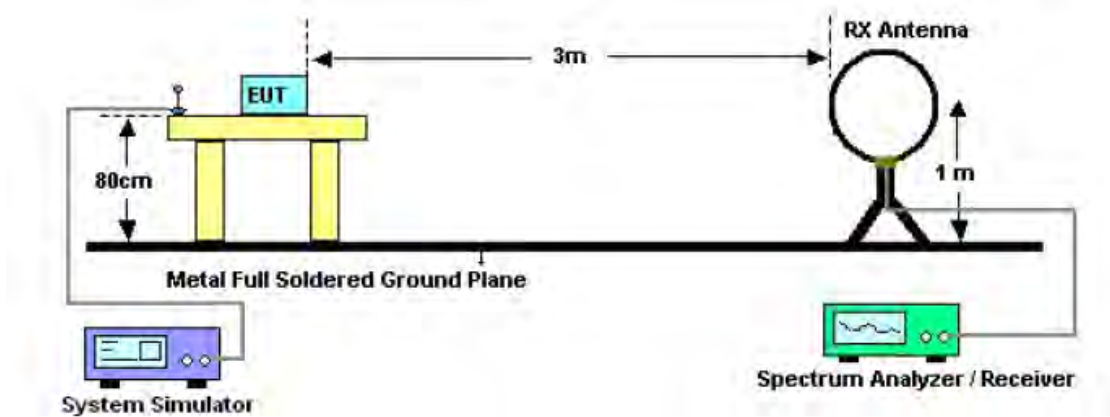
Radiated Emission Test-Setup Frequency Below 30MHz
