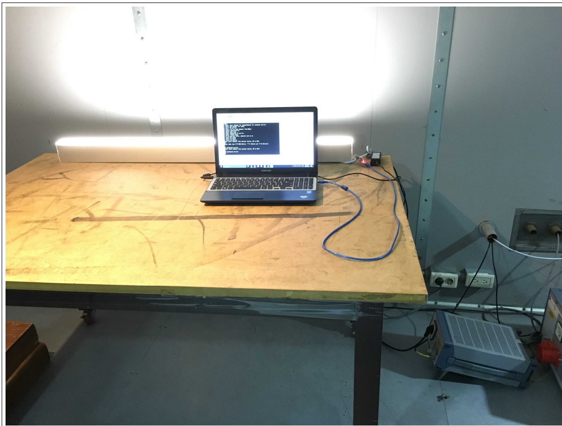
Conducted emission Test
