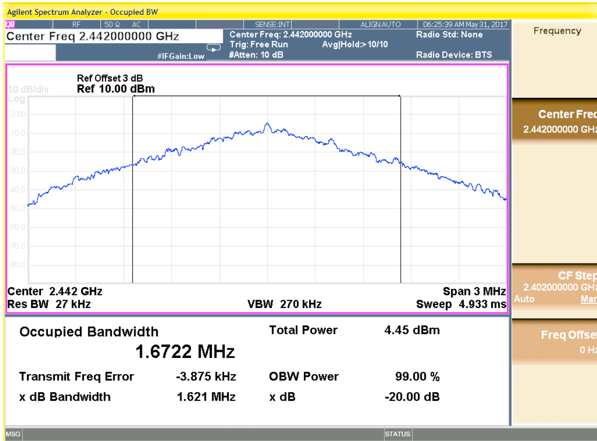
Figure 7: Occupied Bandwidth, Mid Channel
