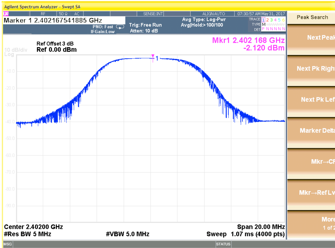
Figure 3: RF Peak Power, Low Channel
