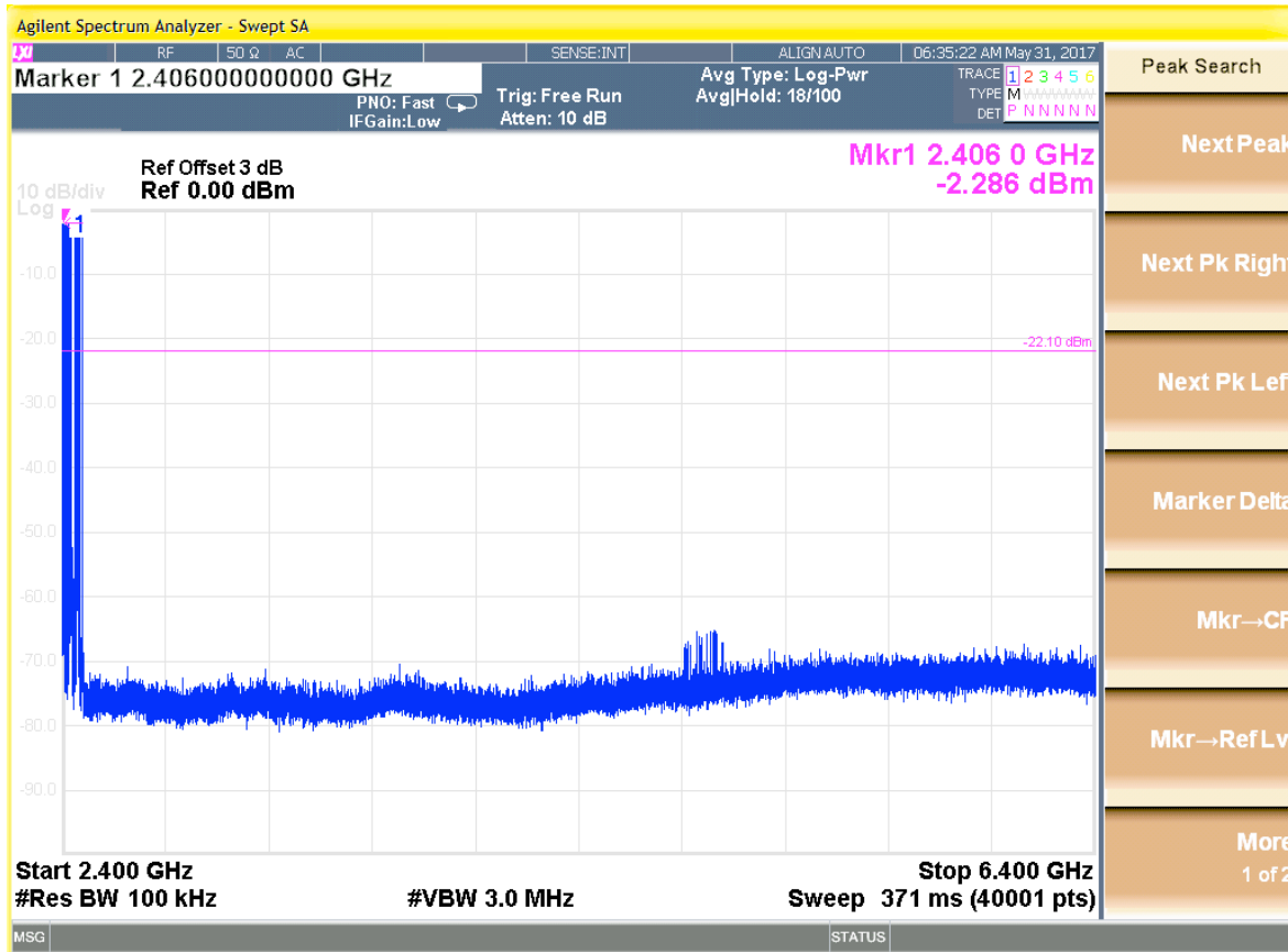
Figure 12: Conducted Spurious Emissions, Channel
