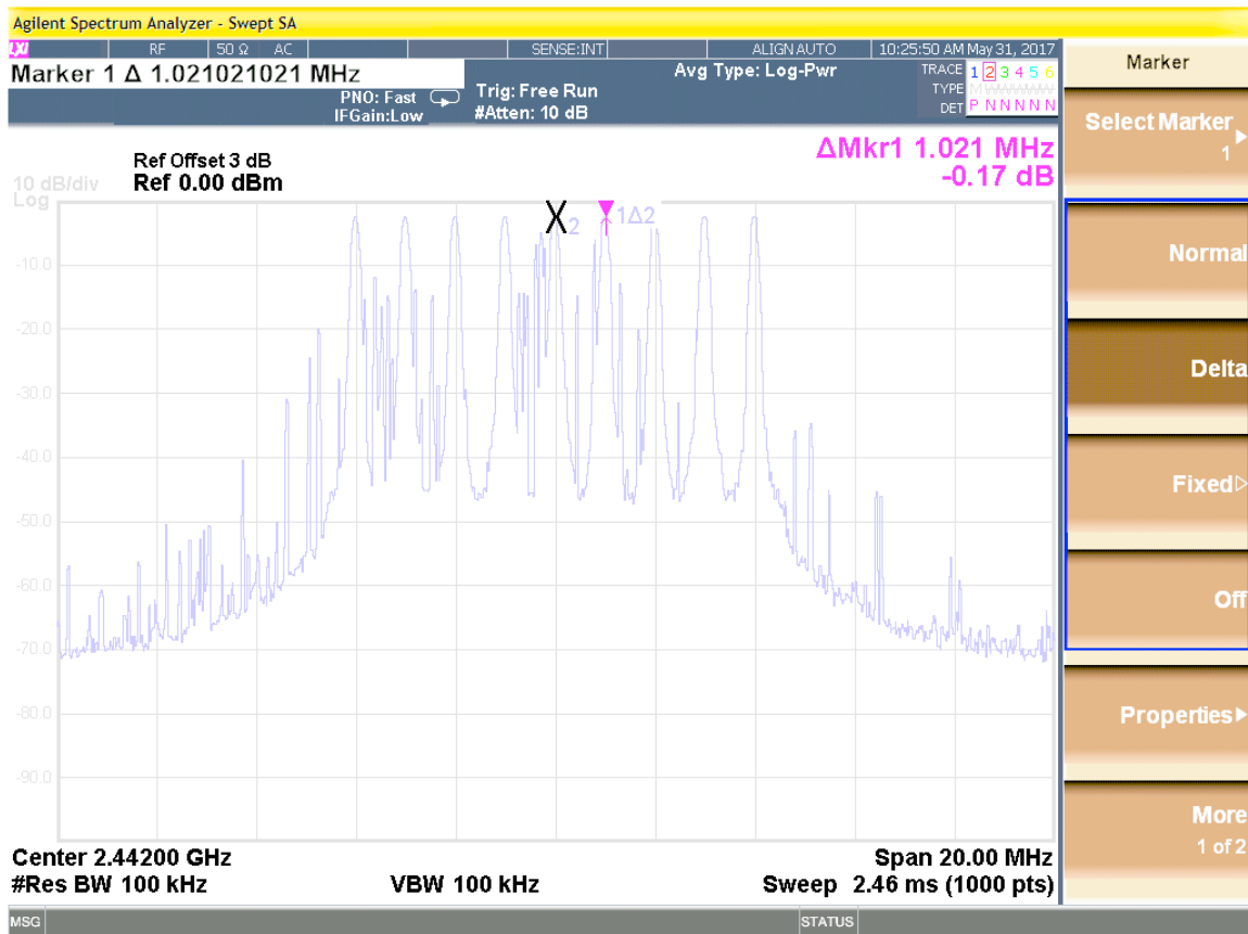
Figure 9: Channel Spacing
