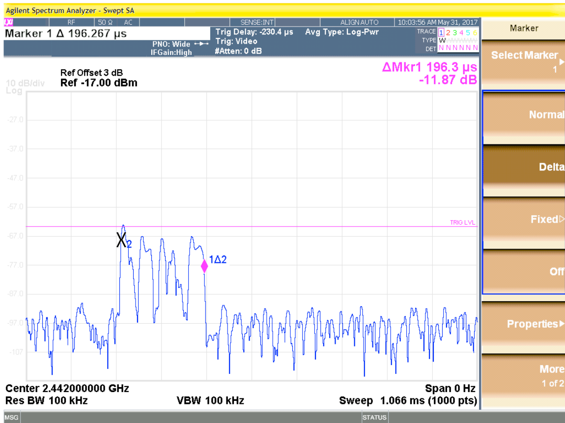
Figure 1: Channel Occupancy
