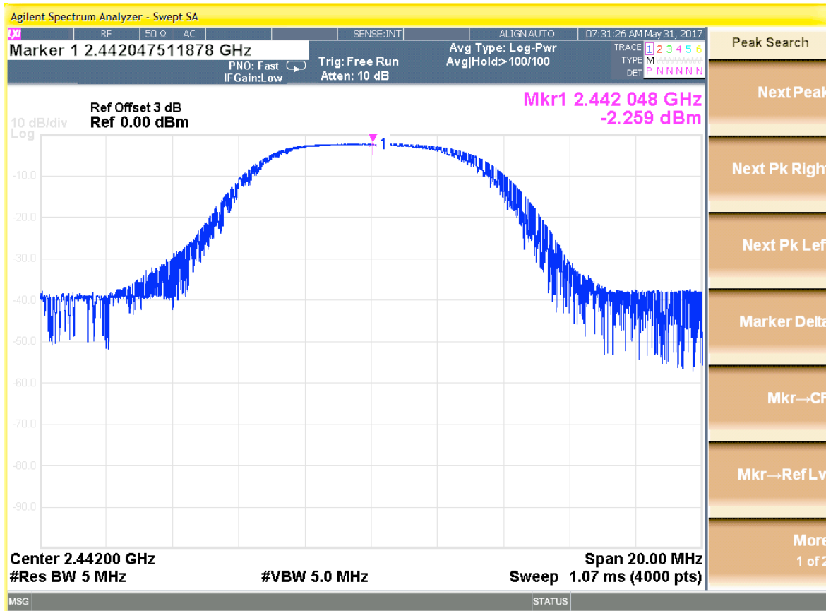
Figure 4: RF Peak Power, Mid Channel
