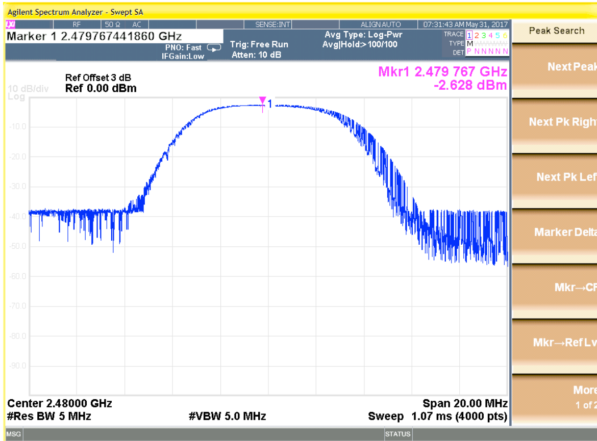
Figure 5: RF Peak Power, High Channel
