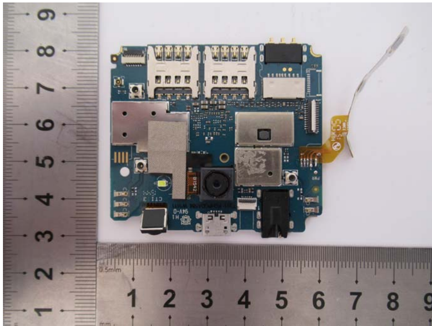
EUT – PCB-2 Shielcing off Bottom View
