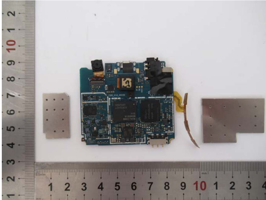
EUT – PCB-2 Shielcing off Top View
