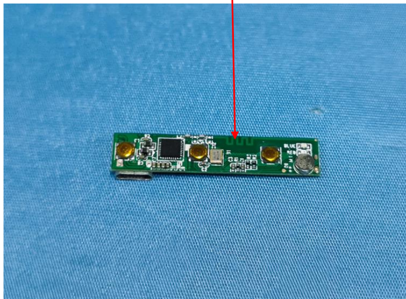
PCB Antenna
