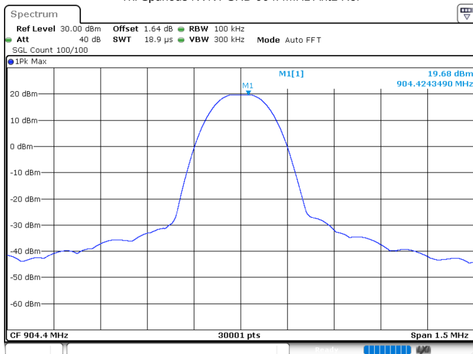
Tx. Spurious NVNT SRD 904.4MHz Ant1 Ref
