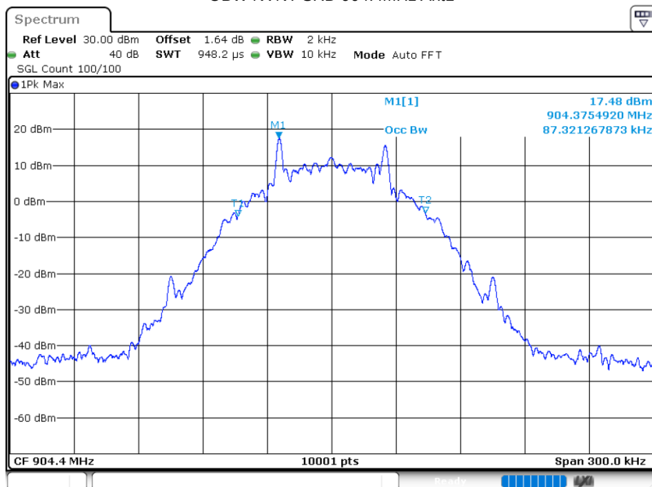
OBW NVNT SRD 904.4MHz Ant1
