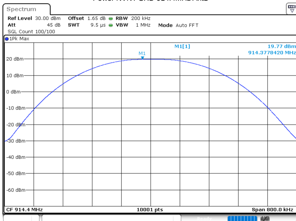
Power NVNT SRD 914.4MHz Ant1
