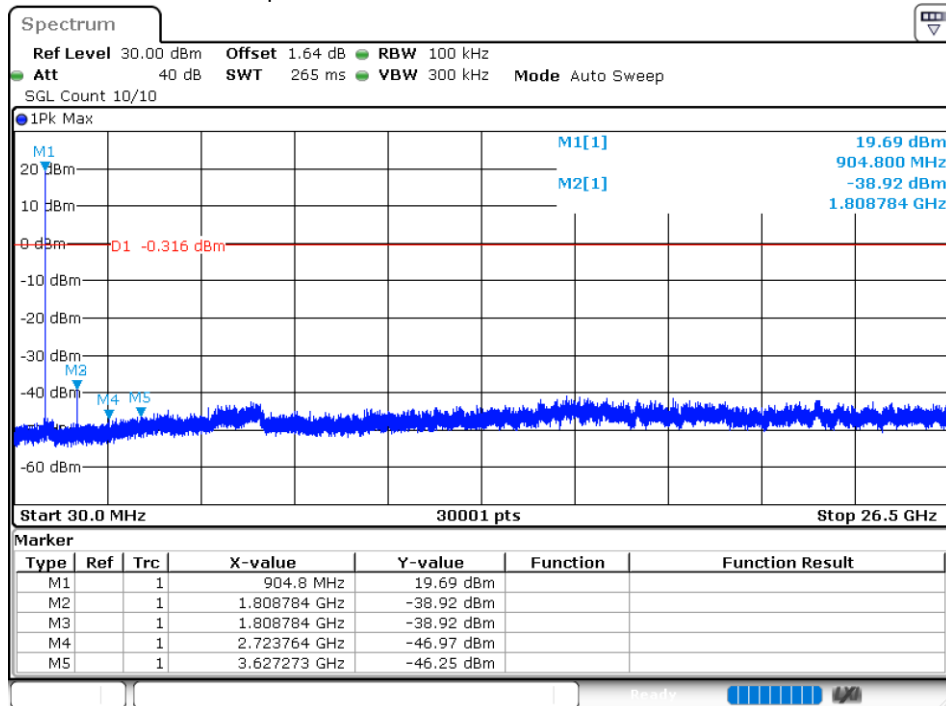
Tx. Spurious NVNT SRD 904.4MHz Ant1 Emission
