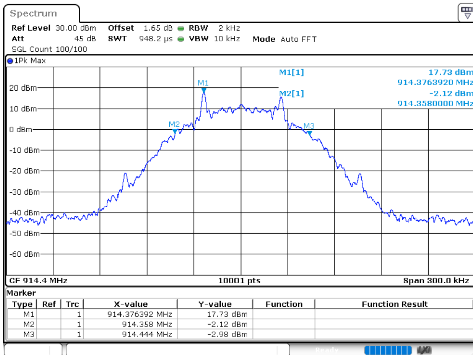
-20dB Bandwidth NVNT SRD 914.4MHz Ant1
