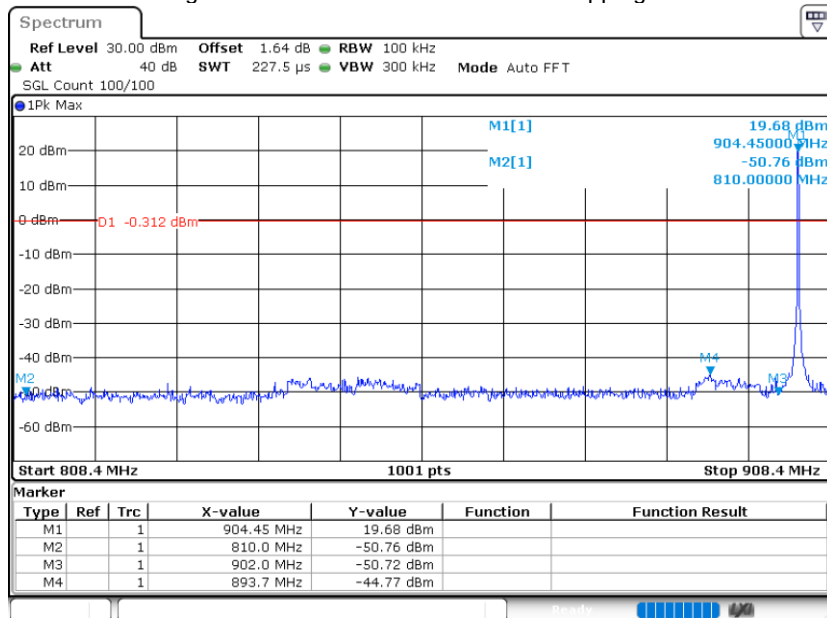
Band Edge NVNT SRD 904.4MHz Ant1 No-Hopping Emission
