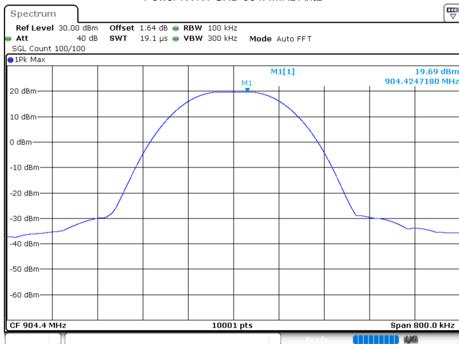
Power NVNT SRD 904.4MHz Ant1
