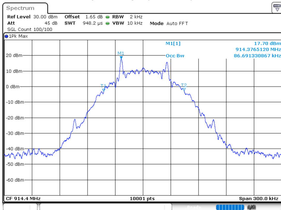
OBW NVNT SRD 914.4MHz Ant1
