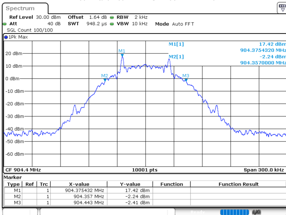
-20dB Bandwidth NVNT SRD 904.4MHz Ant1
