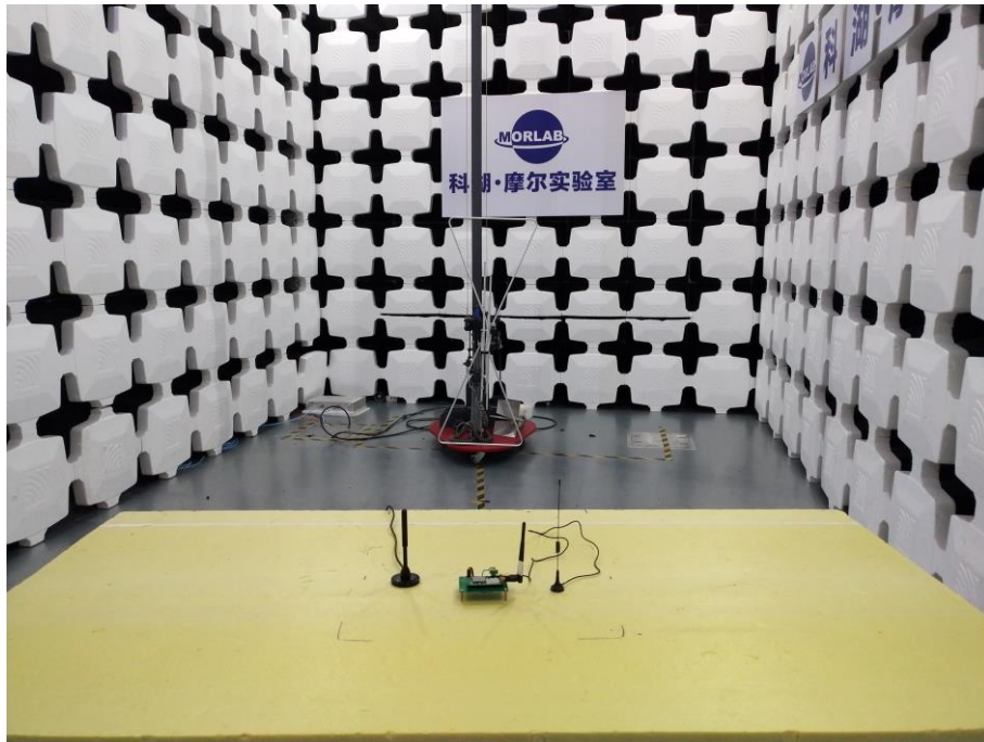
RE Below 1G_ WWAN Link + WiFi Link
