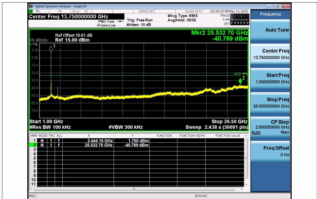
11G-Ant1-2437-1000~26500-PASS
